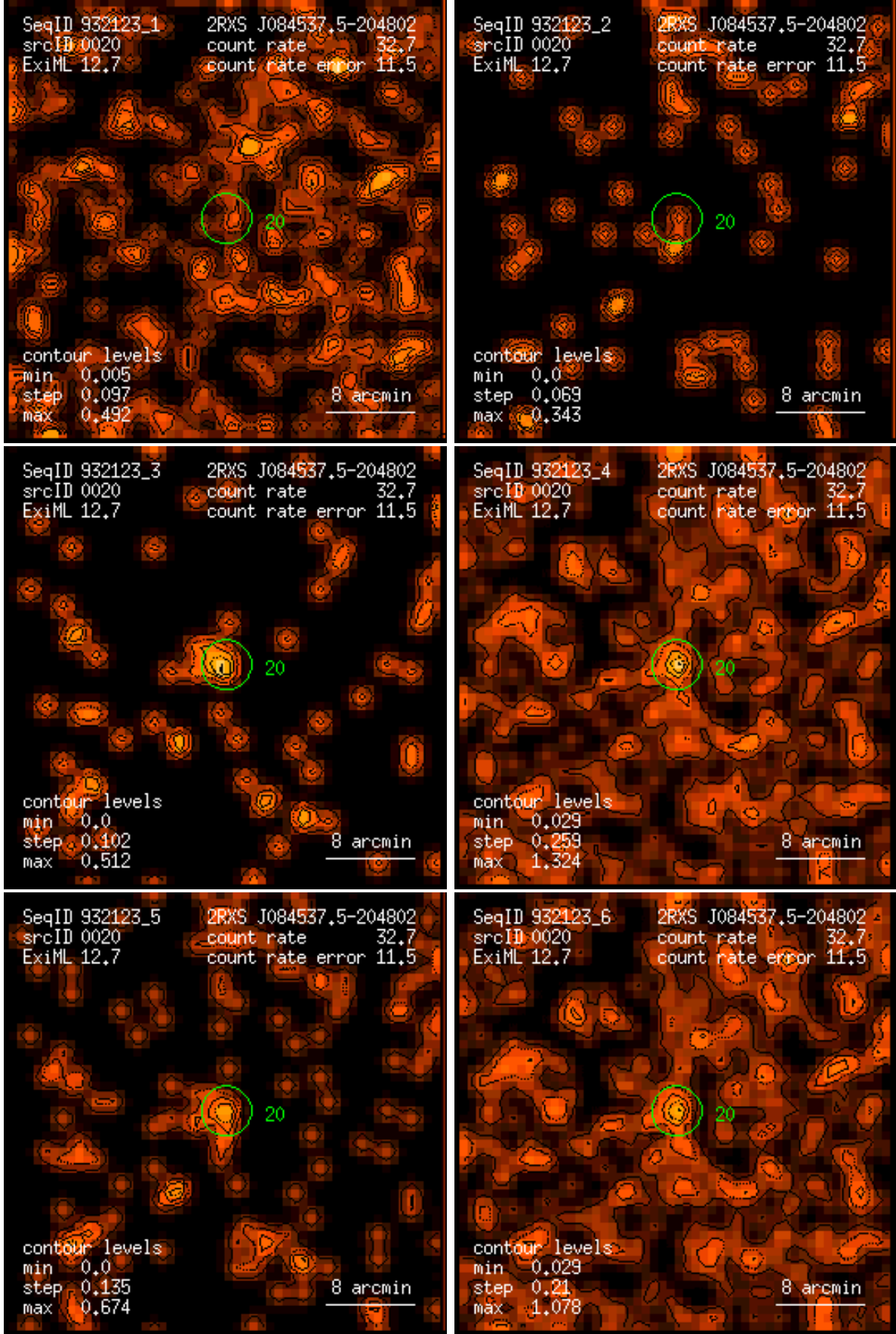
Figure 20: RASS 932123: detection 0020: band rate images, Gaussian filter: (1) PSPC channels 11 – 41, (2) 52 – 90, (3) 91 – 201, (4) 11 – 235, (5) 52 – 201, (6) 11 – 201. Broad band rates in counts/ks. Band rate contour levels in counts/ks/arcmin 2 .
