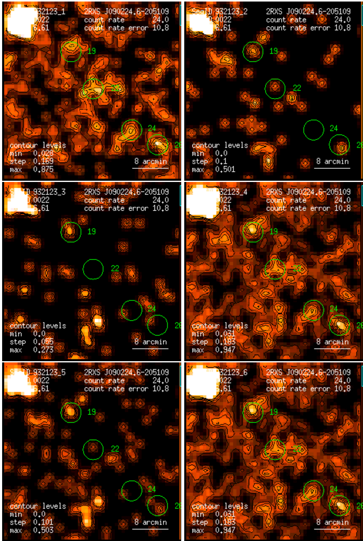
Figure 22: RASS 932123: detection 0022: band rate images, Gaussian filter: (1) PSPC channels 11 – 41, (2) 52 – 90, (3) 91 – 201, (4) 11 – 235, (5) 52 – 201, (6) 11 – 201. Broad band rates in counts/ks. Band rate contour levels in counts/ks/arcmin 2 .
