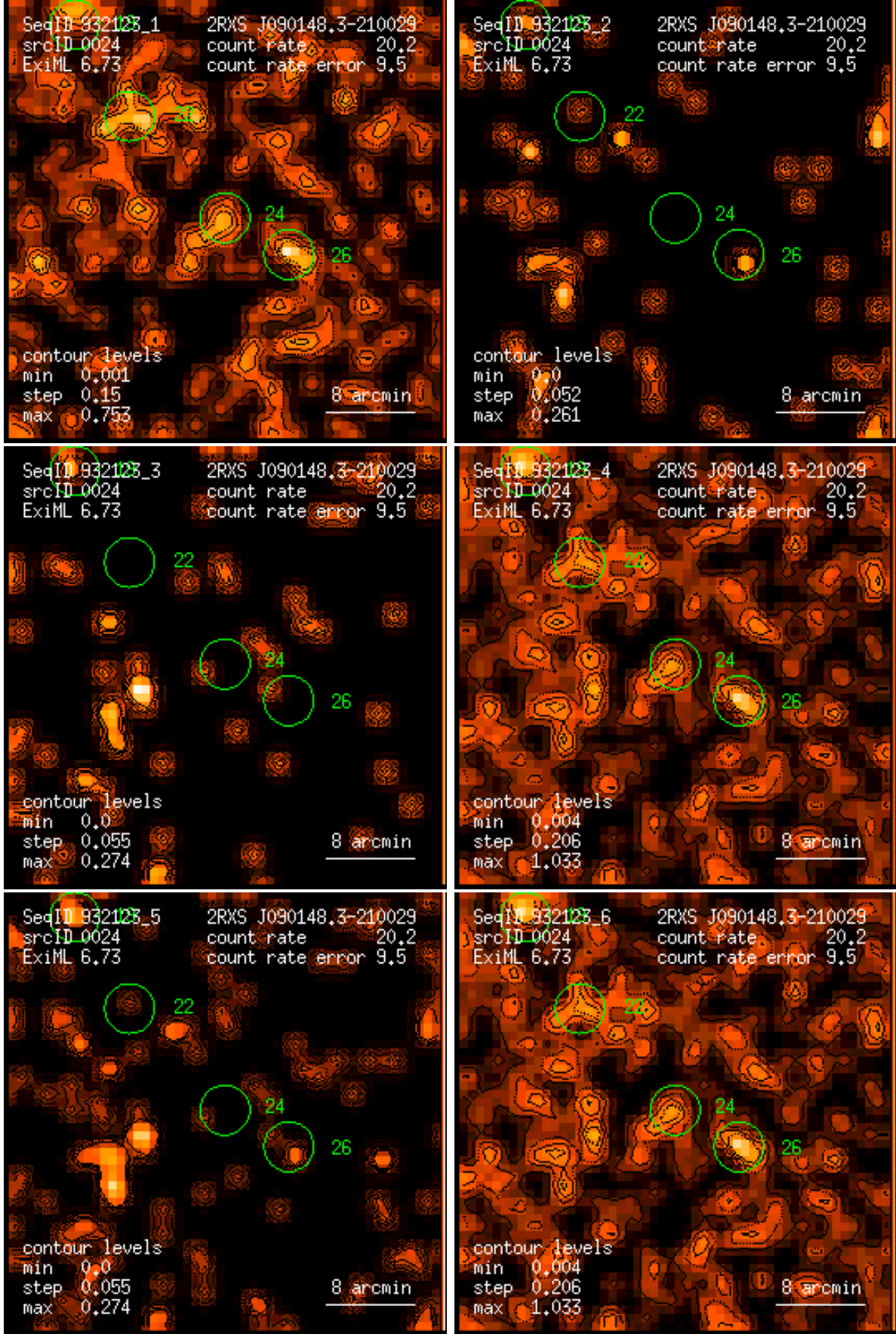
Figure 24: RASS 932123: detection 0024: band rate images, Gaussian filter: (1) PSPC channels 11 – 41, (2) 52 – 90, (3) 91 – 201, (4) 11 – 235, (5) 52 – 201, (6) 11 – 201. Broad band rates in counts/ks. Band rate contour levels in counts/ks/arcmin 2 .
