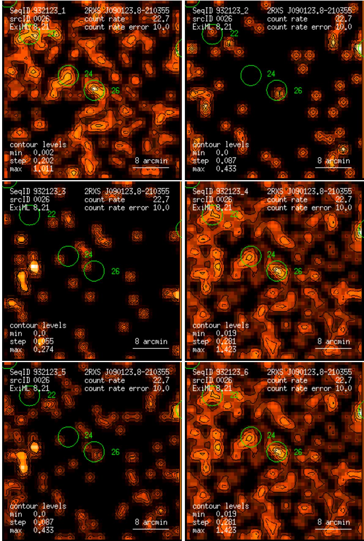
Figure 26: RASS 932123: detection 0026: band rate images, Gaussian filter: (1) PSPC channels 11 – 41, (2) 52 – 90, (3) 91 – 201, (4) 11 – 235, (5) 52 – 201, (6) 11 – 201. Broad band rates in counts/ks. Band rate contour levels in counts/ks/arcmin 2 .
