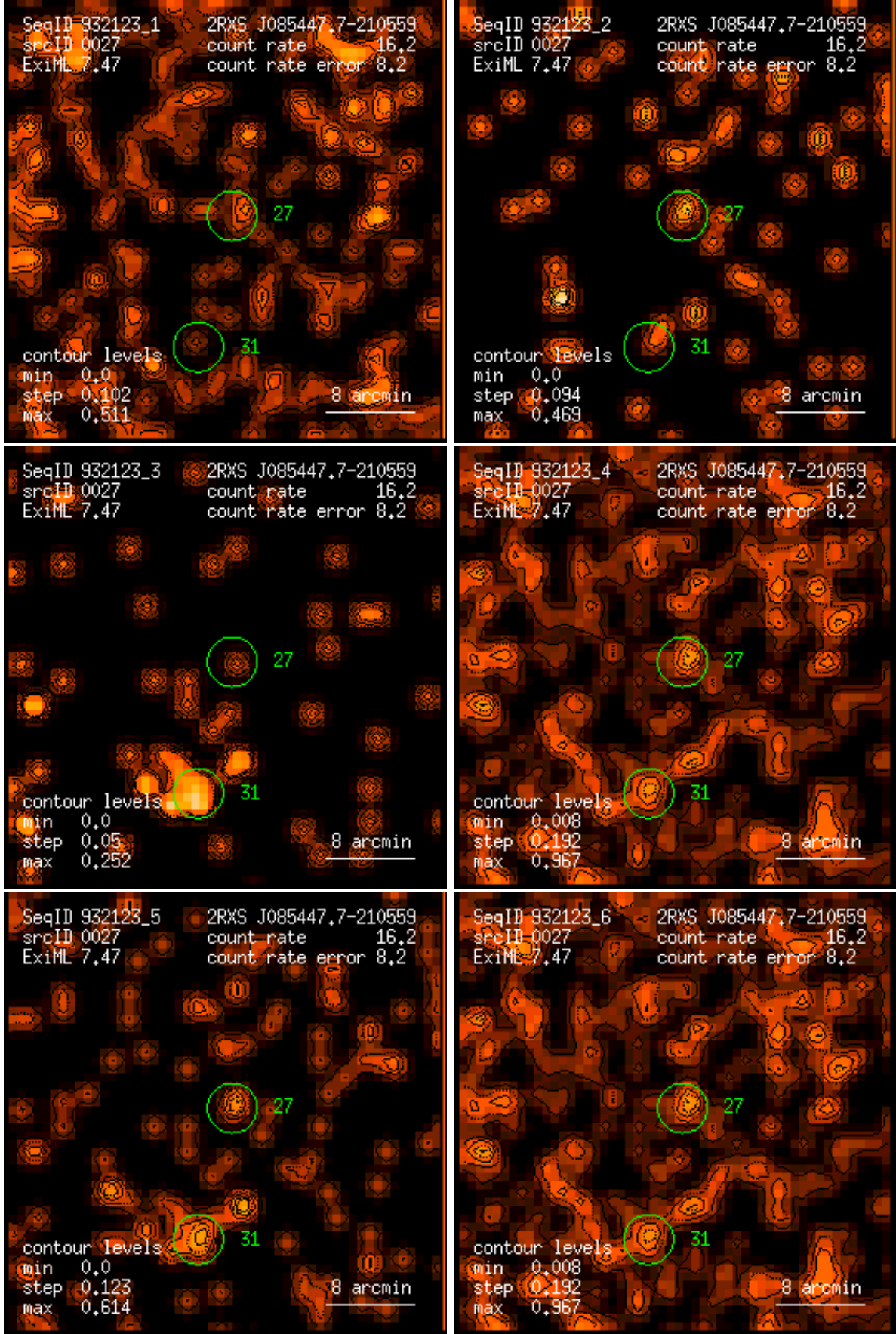
Figure 27: RASS 932123: detection 0027: band rate images, Gaussian filter: (1) PSPC channels 11 – 41, (2) 52 – 90, (3) 91 – 201, (4) 11 – 235, (5) 52 – 201, (6) 11 – 201. Broad band rates in counts/ks. Band rate contour levels in counts/ks/arcmin 2 .
