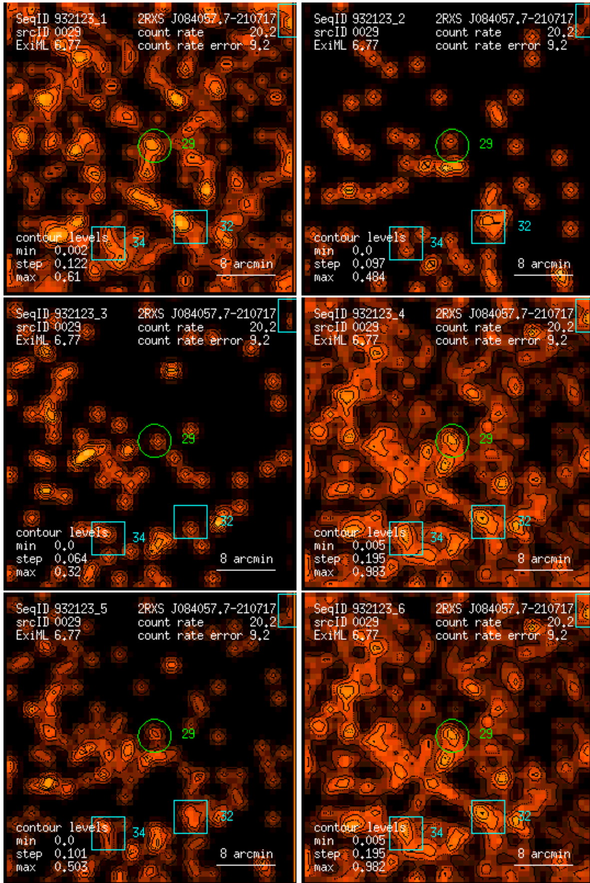
Figure 29: RASS 932123: detection 0029: band rate images, Gaussian filter: (1) PSPC channels 11 – 41, (2) 52 – 90, (3) 91 – 201, (4) 11 – 235, (5) 52 – 201, (6) 11 – 201. Broad band rates in counts/ks. Band rate contour levels in counts/ks/arcmin 2 .
