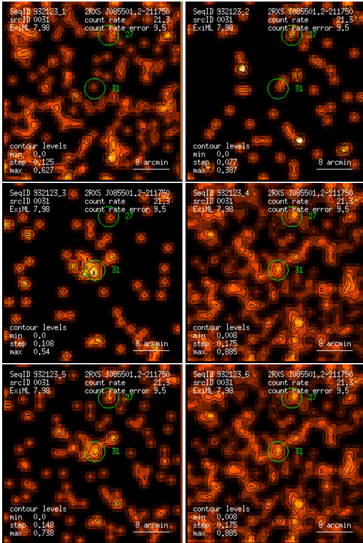
Figure 31: RASS 932123: detection 0031: band rate images, Gaussian filter: (1) PSPC channels 11 – 41, (2) 52 – 90, (3) 91 – 201, (4) 11 – 235, (5) 52 – 201, (6) 11 – 201. Broad band rates in counts/ks. Band rate contour levels in counts/ks/arcmin 2 .
