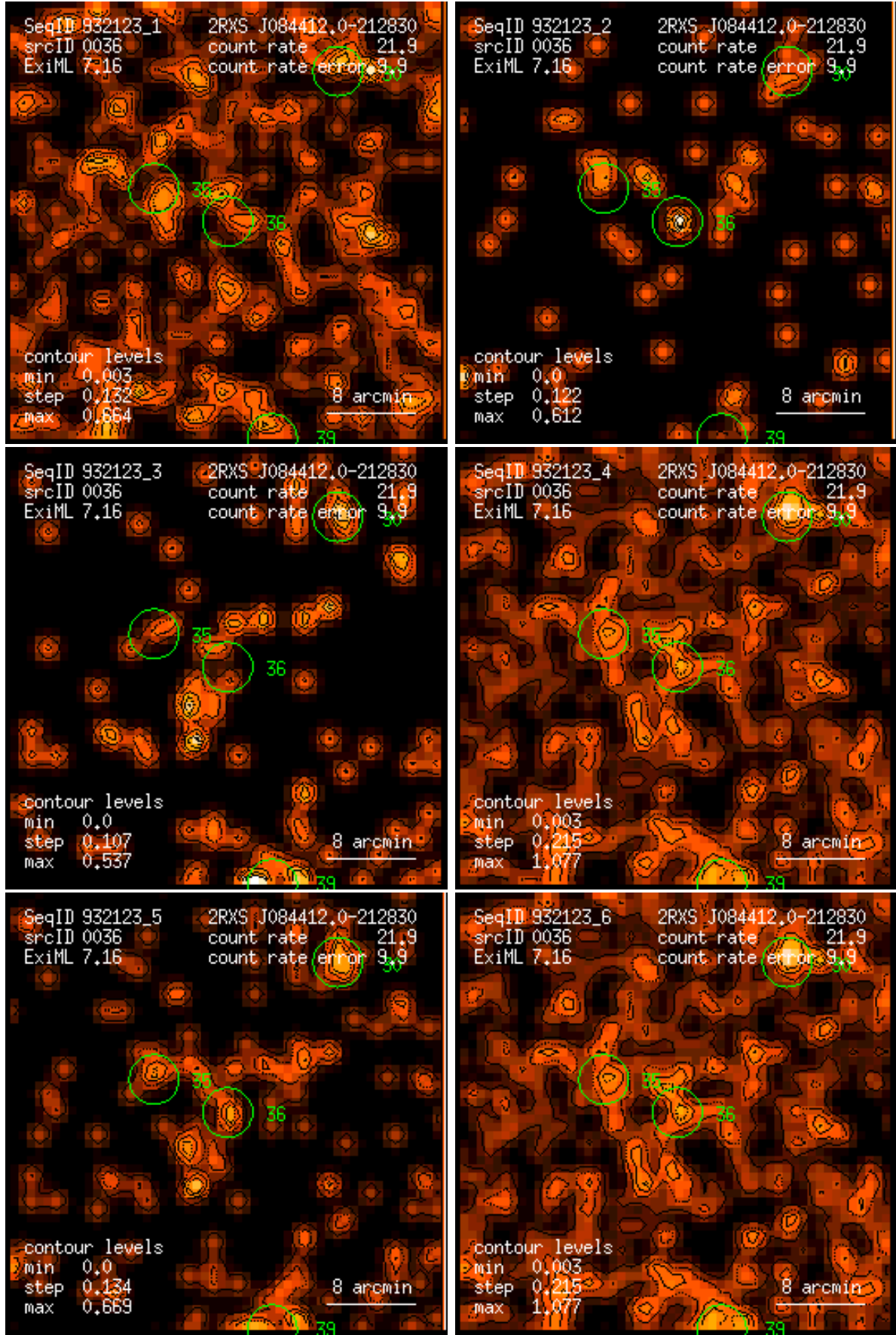
Figure 36: RASS 932123: detection 0036: band rate images, Gaussian filter: (1) PSPC channels 11 – 41, (2) 52 – 90, (3) 91 – 201, (4) 11 – 235, (5) 52 – 201, (6) 11 – 201. Broad band rates in counts/ks. Band rate contour levels in counts/ks/arcmin 2 .
