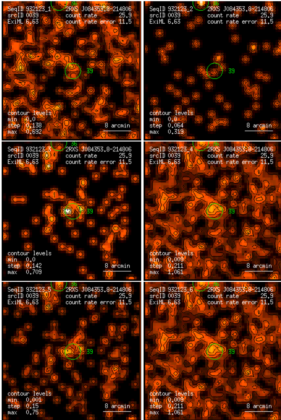
Figure 39: RASS 932123: detection 0039: band rate images, Gaussian filter: (1) PSPC channels 11 – 41, (2) 52 – 90, (3) 91 – 201, (4) 11 – 235, (5) 52 – 201, (6) 11 – 201. Broad band rates in counts/ks. Band rate contour levels in counts/ks/arcmin 2 .
