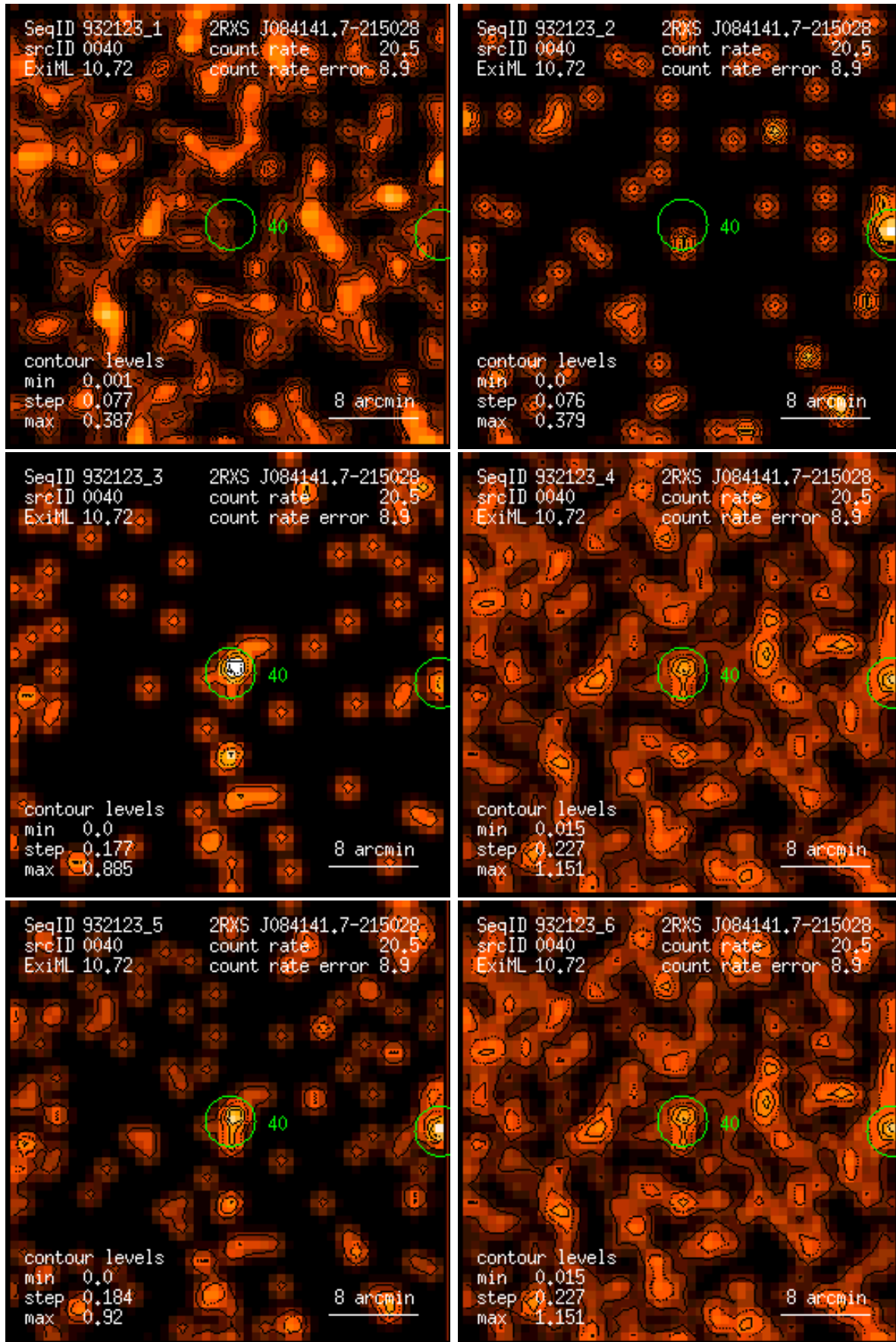
Figure 40: RASS 932123: detection 0040: band rate images, Gaussian filter: (1) PSPC channels 11 – 41, (2) 52 – 90, (3) 91 – 201, (4) 11 – 235, (5) 52 – 201, (6) 11 – 201. Broad band rates in counts/ks. Band rate contour levels in counts/ks/arcmin 2 .
