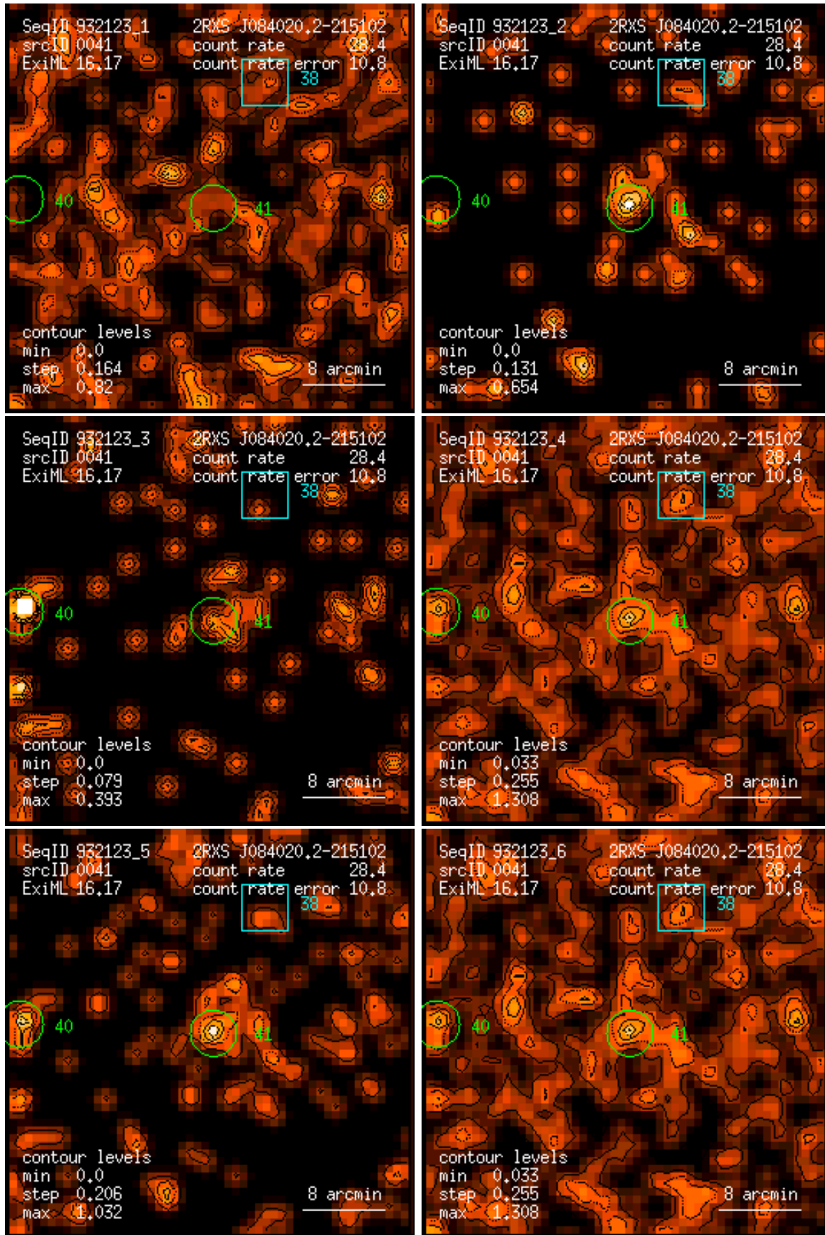
Figure 41: RASS 932123: detection 0041: band rate images, Gaussian filter: (1) PSPC channels 11 – 41, (2) 52 – 90, (3) 91 – 201, (4) 11 – 235, (5) 52 – 201, (6) 11 – 201. Broad band rates in counts/ks. Band rate contour levels in counts/ks/arcmin 2 .
