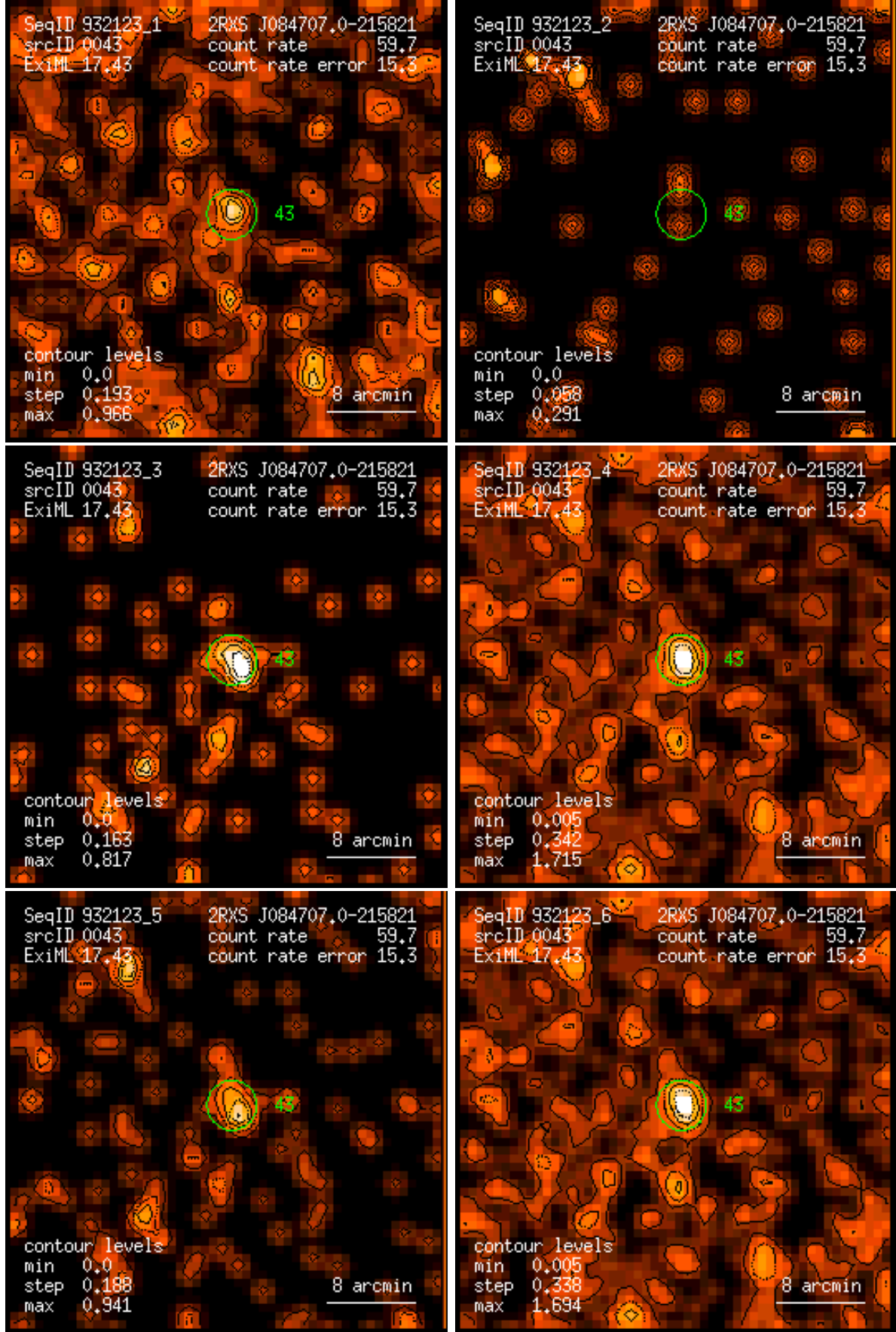
Figure 43: RASS 932123: detection 0043: band rate images, Gaussian filter: (1) PSPC channels 11 – 41, (2) 52 – 90, (3) 91 – 201, (4) 11 – 235, (5) 52 – 201, (6) 11 – 201. Broad band rates in counts/ks. Band rate contour levels in counts/ks/arcmin 2 .
