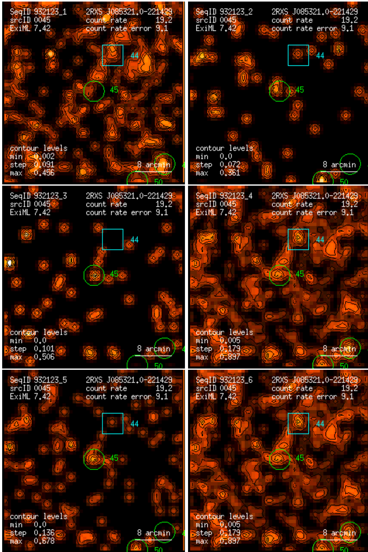
Figure 45: RASS 932123: detection 0045: band rate images, Gaussian filter: (1) PSPC channels 11 – 41, (2) 52 – 90, (3) 91 – 201, (4) 11 – 235, (5) 52 – 201, (6) 11 – 201. Broad band rates in counts/ks. Band rate contour levels in counts/ks/arcmin 2 .
