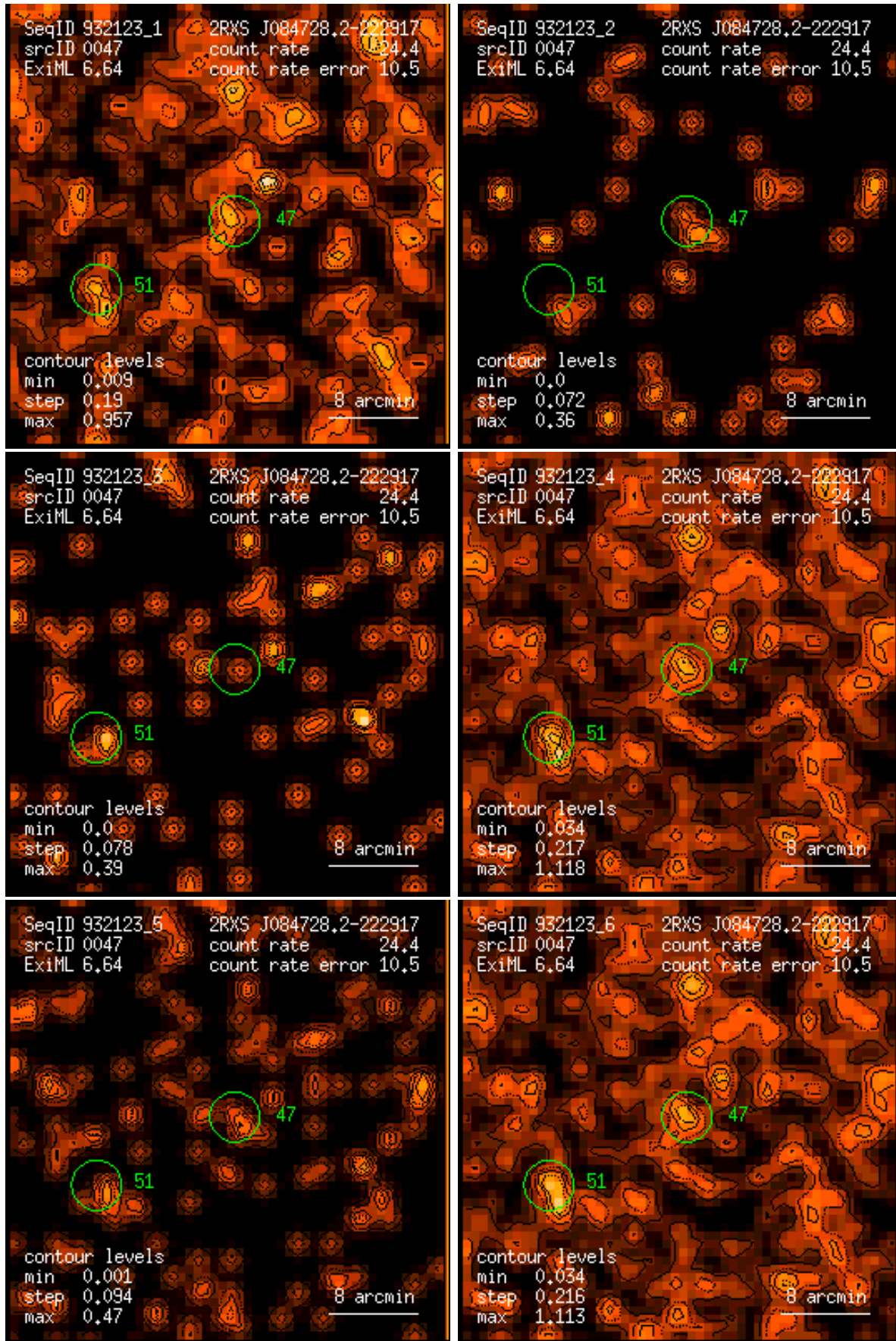
Figure 47: RASS 932123: detection 0047: band rate images, Gaussian filter: (1) PSPP channels 11 – 41, (2) 52 – 90, (3) 91 – 201, (4) 11 – 235, (5) 52 – 201, (6) 11 – 201. Broad band rates in counts/ks. Band rate contour levels in counts/ks/arcmin 2 .
