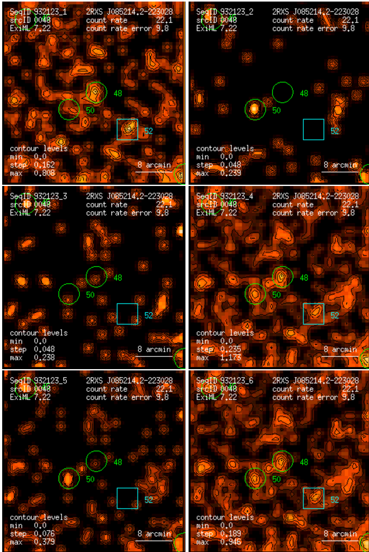
Figure 48: RASS 932123: detection 0048: band rate images, Gaussian filter: (1) PSPC channels 11 – 41, (2) 52 – 90, (3) 91 – 201, (4) 11 – 235, (5) 52 – 201, (6) 11 – 201. Broad band rates in counts/ks. Band rate contour levels in counts/ks/arcmin 2 .
