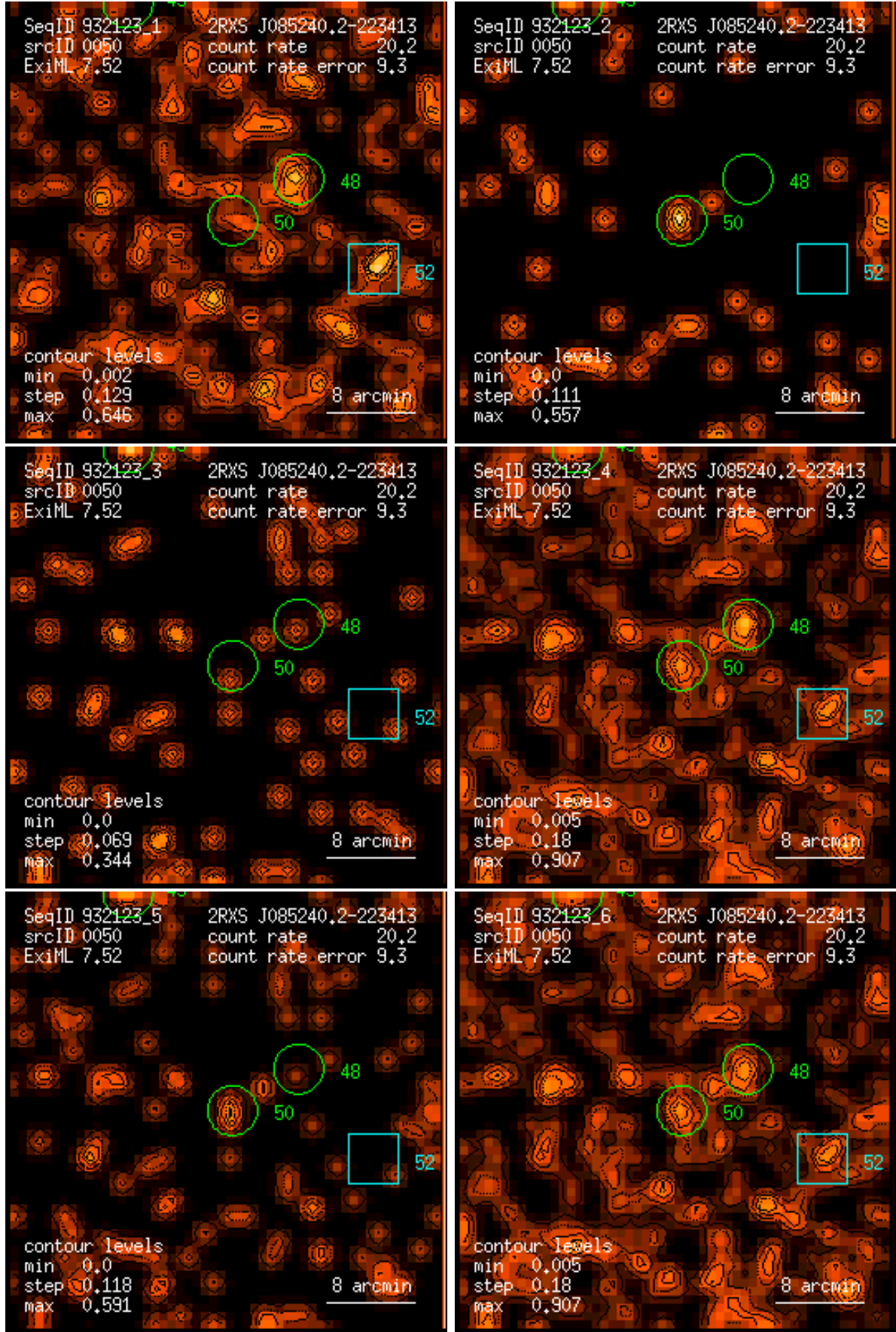
Figure 50: RASS 932123: detection 0050: band rate images, Gaussian filter: (1) PSPC channels 11 – 41, (2) 52 – 90, (3) 91 – 201, (4) 11 – 235, (5) 52 – 201, (6) 11 – 201. Broad band rates in counts/ks. Band rate contour levels in counts/ks/arcmin 2 .
