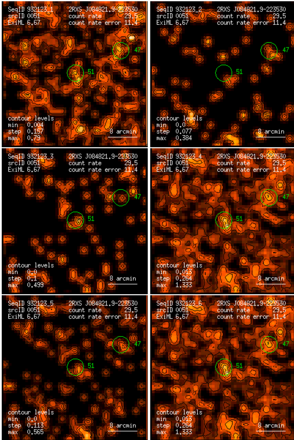
Figure 51: RASS 932123: detection 0051: band rate images, Gaussian filter: (1) PSPC channels 11 – 41, (2) 52 – 90, (3) 91 – 201, (4) 11 – 235, (5) 52 – 201, (6) 11 – 201. Broad band rates in counts/ks. Band rate contour levels in counts/ks/arcmin 2 .
