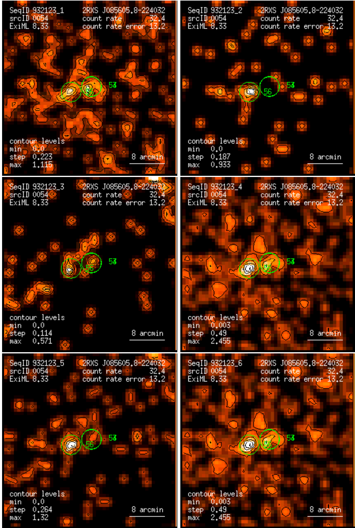
Figure 54: RASS 932123: detection 0054: band rate images, Gaussian filter: (1) PSPC channels 11 – 41, (2) 52 – 90, (3) 91 – 201, (4) 11 – 235, (5) 52 – 201, (6) 11 – 201. Broad band rates in counts/ks. Band rate contour levels in counts/ks/arcmin 2 .
