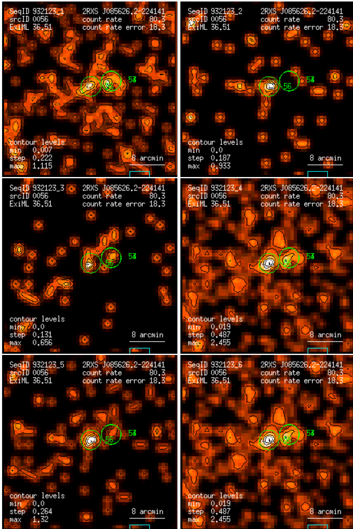
Figure 56: RASS 932123: detection 0056: band rate images, Gaussian filter: (1) PSPC channels 11 – 41, (2) 52 – 90, (3) 91 – 201, (4) 11 – 235, (5) 52 – 201, (6) 11 – 201. Broad band rates in counts/ks. Band rate contour levels in counts/ks/arcmin 2 .
