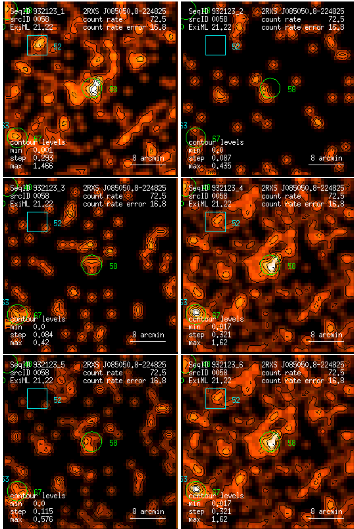
Figure 58: RASS 932123: detection 0058: band rate images, Gaussian filter: (1) PSPC channels 11 – 41, (2) 52 – 90, (3) 91 – 201, (4) 11 – 235, (5) 52 – 201, (6) 11 – 201. Broad band rates in counts/ks. Band rate contour levels in counts/ks/arcmin 2 .
