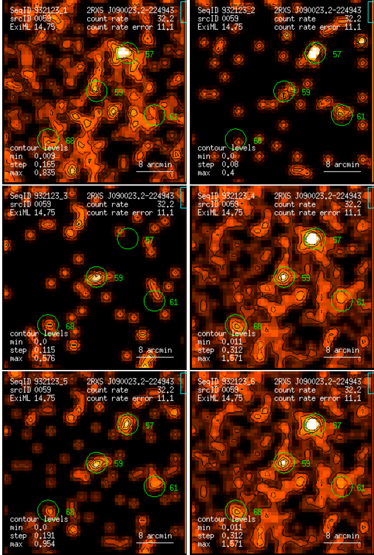
Figure 59: RASS 932123: detection 0059: band rate images, Gaussian filter: (1) PSPC channels 11 – 41, (2) 52 – 90, (3) 91 – 201, (4) 11 – 235, (5) 52 – 201, (6) 11 – 201. Broad band rates in counts/ks. Band rate contour levels in counts/ks/arcmin 2 .
