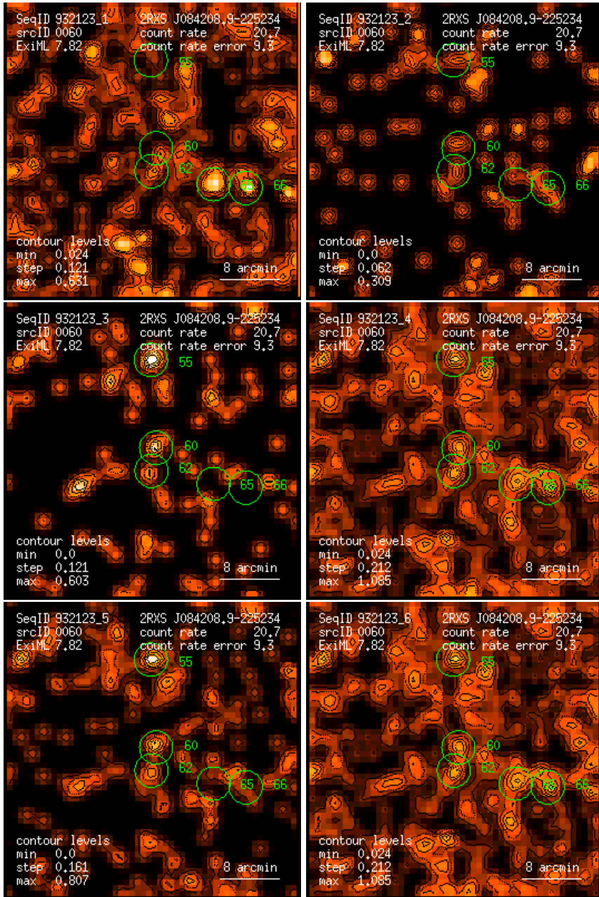
Figure 60: RASS 932123: detection 0060: band rate images, Gaussian filter: (1) PSPC channels 11 – 41, (2) 52 – 90, (3) 91 – 201, (4) 11 – 235, (5) 52 – 201, (6) 11 – 201. Broad band rates in counts/ks. Band rate contour levels in counts/ks/arcmin 2 .
