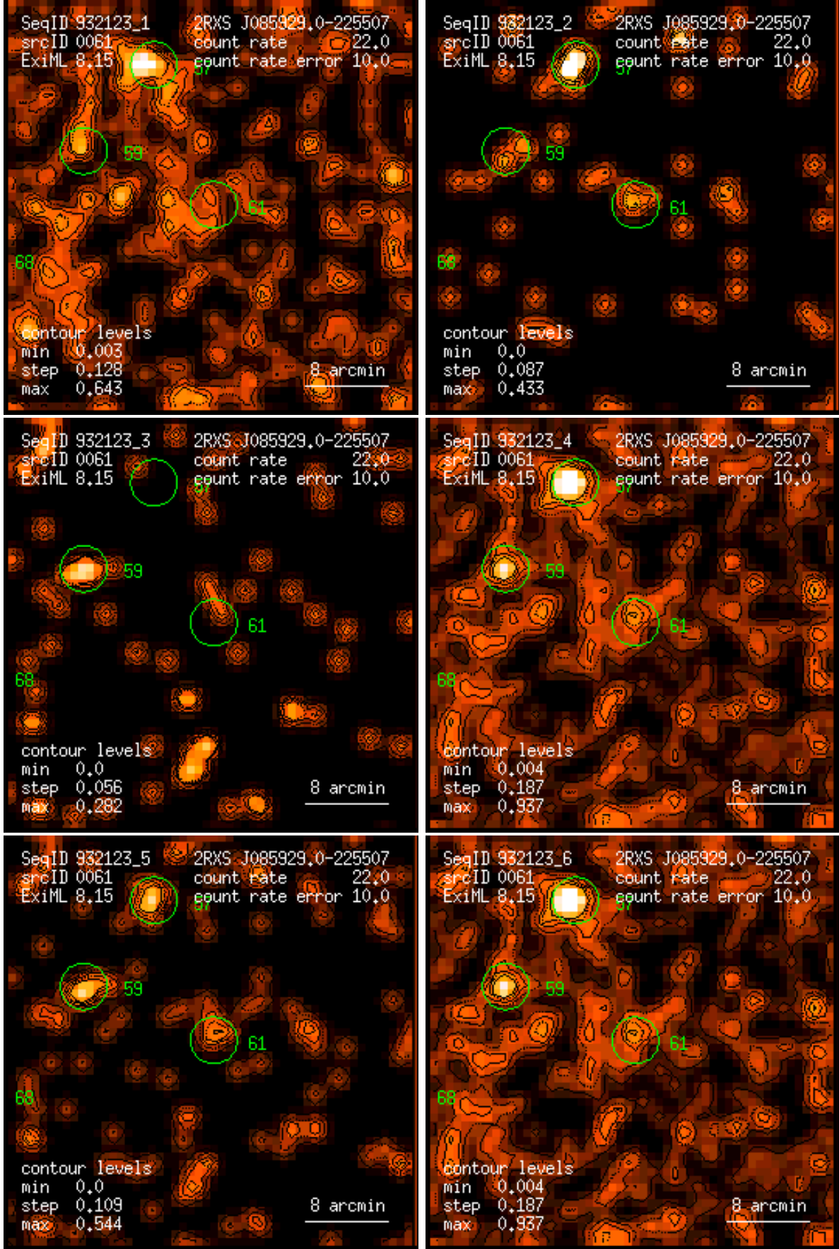
Figure 61: RASS 932123: detection 0061: band rate images, Gaussian filter: (1) PSPC channels 11 – 41, (2) 52 – 90, (3) 91 – 201, (4) 11 – 235, (5) 52 – 201, (6) 11 – 201. Broad band rates in counts/ks. Band rate contour levels in counts/ks/arcmin 2 .
