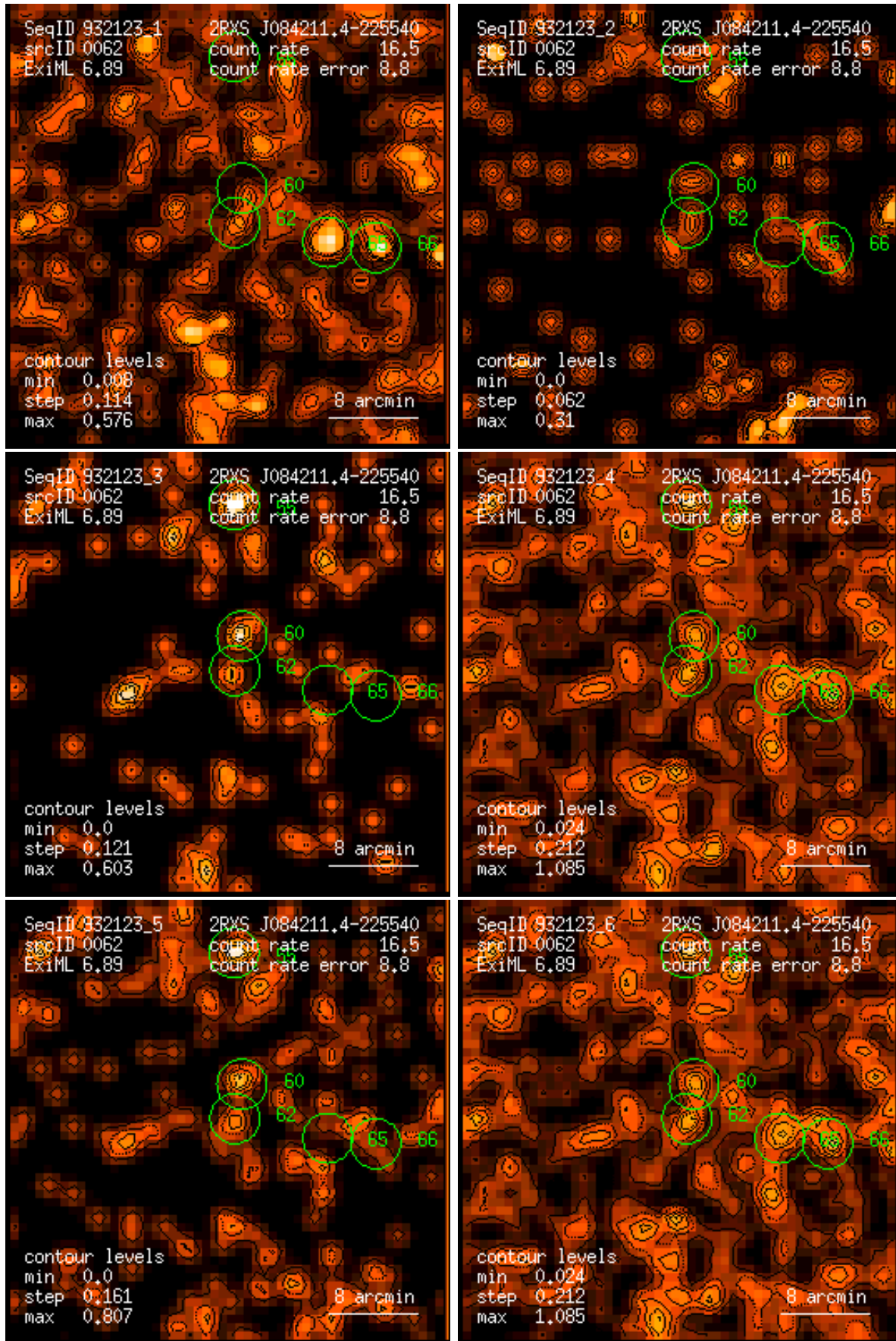
Figure 62: RASS 932123: detection 0062: band rate images, Gaussian filter: (1) PSPC channels 11 – 41, (2) 52 – 90, (3) 91 – 201, (4) 11 – 235, (5) 52 – 201, (6) 11 – 201. Broad band rates in counts/ks. Band rate contour levels in counts/ks/arcmin 2 .
