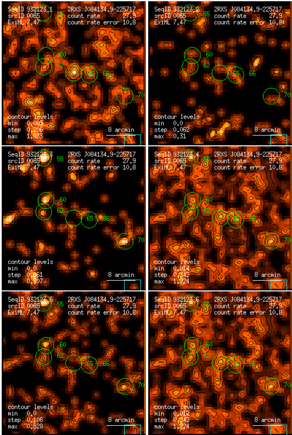
Figure 65: RASS 932123: detection 0065: band rate images, Gaussian filter: (1) PSPC channels 11 – 41, (2) 52 – 90, (3) 91 – 201, (4) 11 – 235, (5) 52 – 201, (6) 11 – 201. Broad band rates in counts/ks. Band rate contour levels in counts/ks/arcmin 2 .
