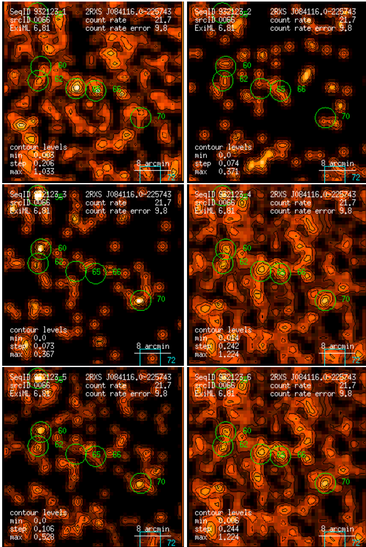
Figure 66: RASS 932123: detection 0066: band rate images, Gaussian filter: (1) PSPC channels 11 – 41, (2) 52 – 90, (3) 91 – 201, (4) 11 – 235, (5) 52 – 201, (6) 11 – 201. Broad band rates in counts/ks. Band rate contour levels in counts/ks/arcmin 2 .
