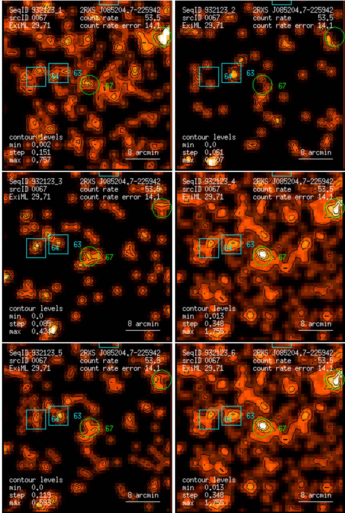
Figure 67: RASS 932123: detection 0067: band rate images, Gaussian filter: (1) PSPC channels 11 – 41, (2) 52 – 90, (3) 91 – 201, (4) 11 – 235, (5) 52 – 201, (6) 11 – 201. Broad band rates in counts/ks. Band rate contour levels in counts/ks/arcmin 2 .
