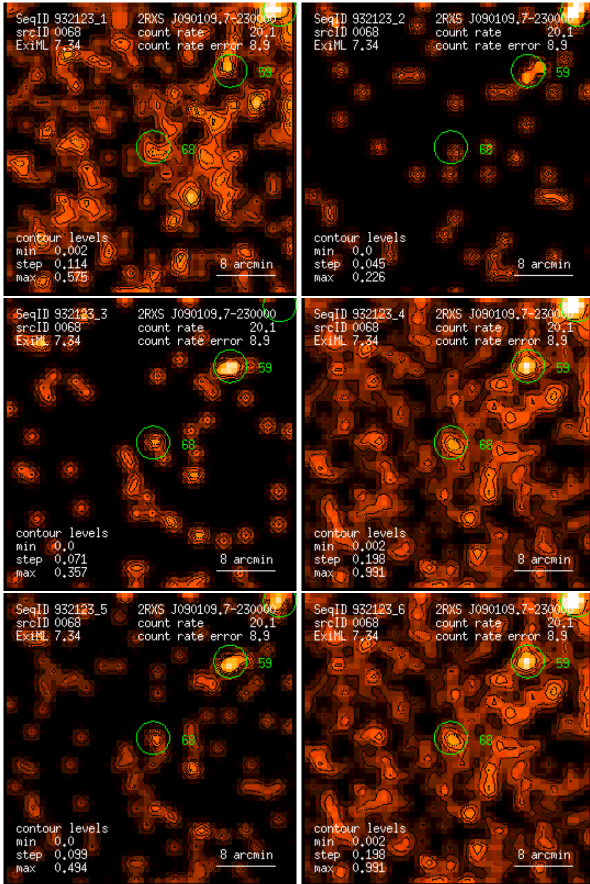
Figure 68: RASS 932123: detection 0068: band rate images, Gaussian filter: (1) PSPC channels 11 – 41, (2) 52 – 90, (3) 91 – 201, (4) 11 – 235, (5) 52 – 201, (6) 11 – 201. Broad band rates in counts/ks. Band rate contour levels in counts/ks/arcmin 2 .
