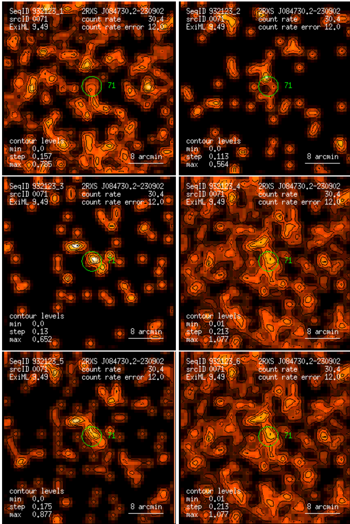
Figure 71: RASS 932123: detection 0071: band rate images, Gaussian filter: (1) PSPC channels 11 – 41, (2) 52 – 90, (3) 91 – 201, (4) 11 – 235, (5) 52 – 201, (6) 11 – 201. Broad band rates in counts/ks. Band rate contour levels in counts/ks/arcmin 2 .
