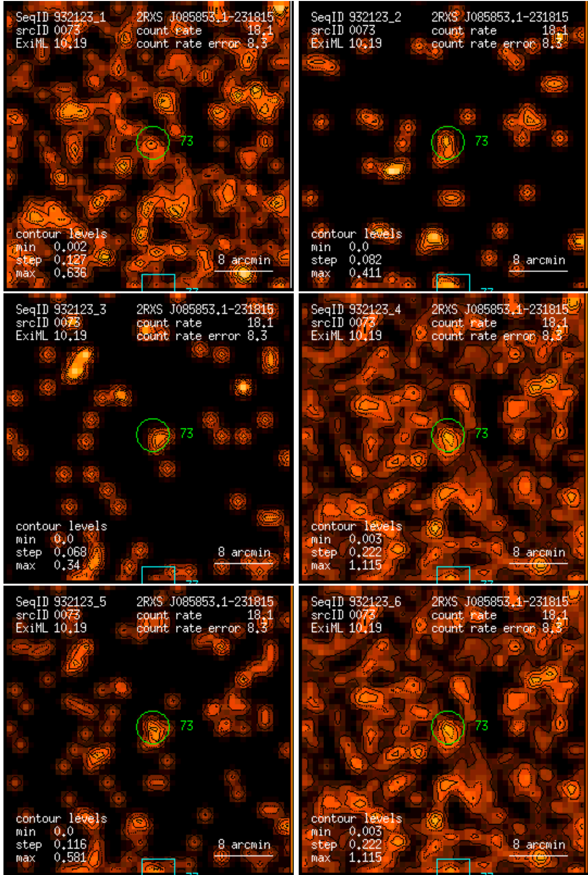
Figure 73: RASS 932123: detection 0073: band rate images, Gaussian filter: (1) PSPC channels 11 – 41, (2) 52 – 90, (3) 91 – 201, (4) 11 – 235, (5) 52 – 201, (6) 11 – 201. Broad band rates in counts/ks. Band rate contour levels in counts/ks/arcmin 2 .
