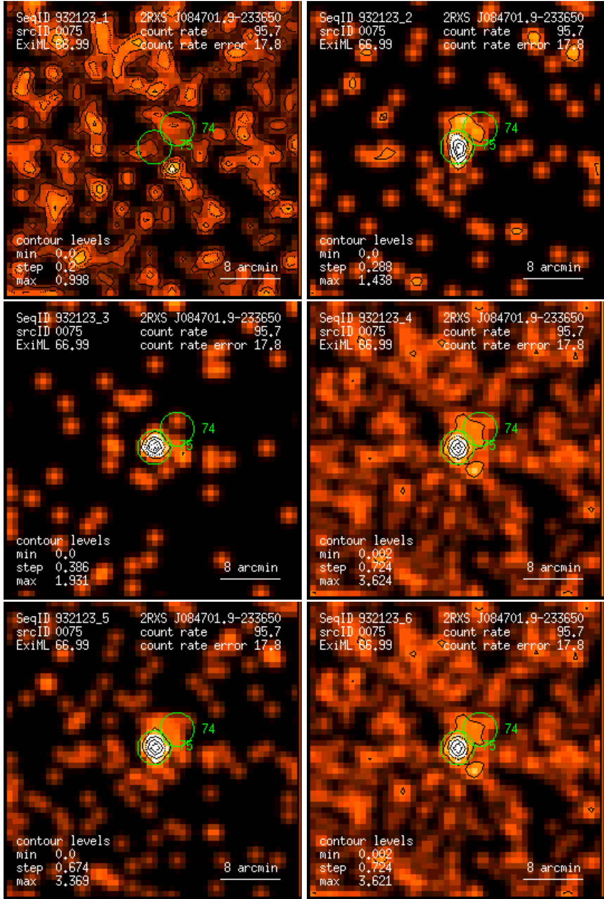
Figure 75: RASS 932123: detection 0075: band rate images, Gaussian filter: (1) PSPC channels 11 – 41, (2) 52 – 90, (3) 91 – 201, (4) 11 – 235, (5) 52 – 201, (6) 11 – 201. Broad band rates in counts/ks. Band rate contour levels in counts/ks/arcmin 2 .
