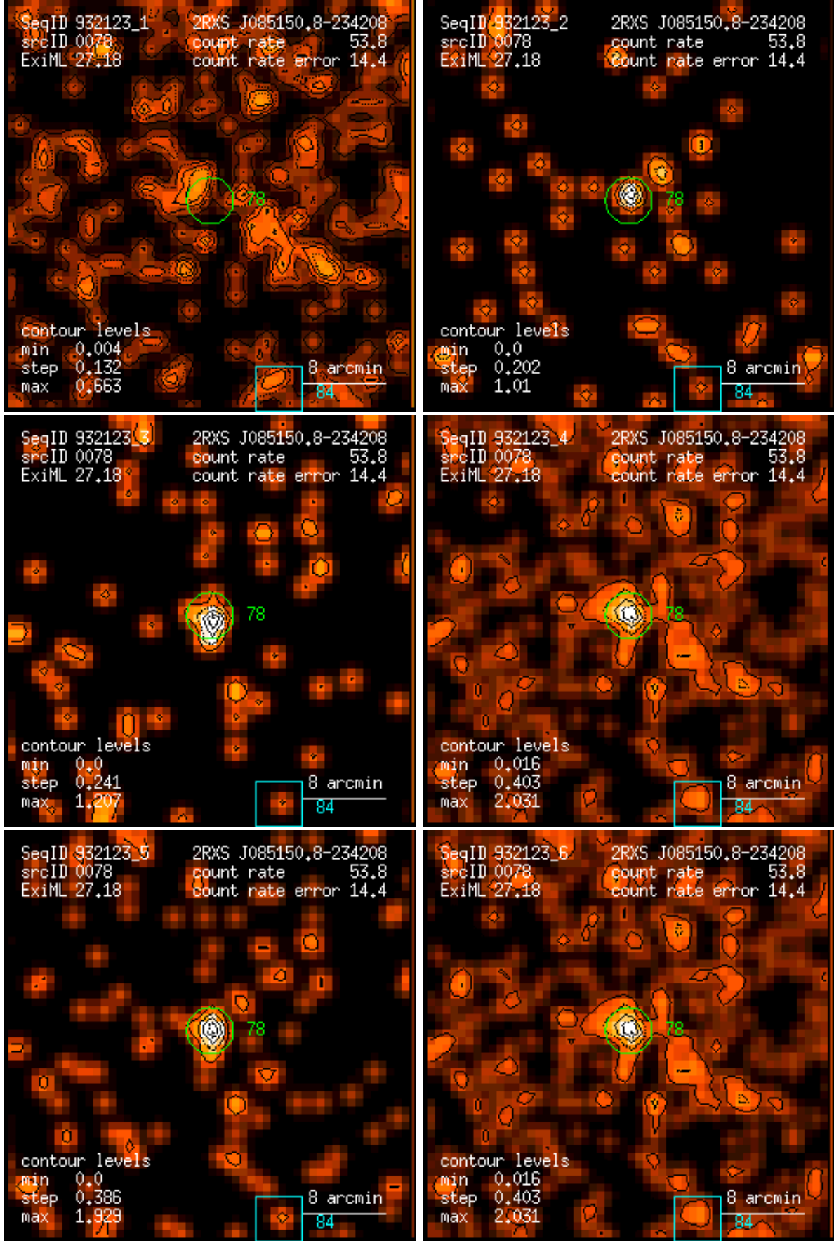
Figure 78: RASS 932123: detection 0078: band rate images, Gaussian filter: (1) PSPC channels 11 – 41, (2) 52 – 90, (3) 91 – 201, (4) 11 – 235, (5) 52 – 201, (6) 11 – 201. Broad band rates in counts/ks. Band rate contour levels in counts/ks/arcmin 2 .
