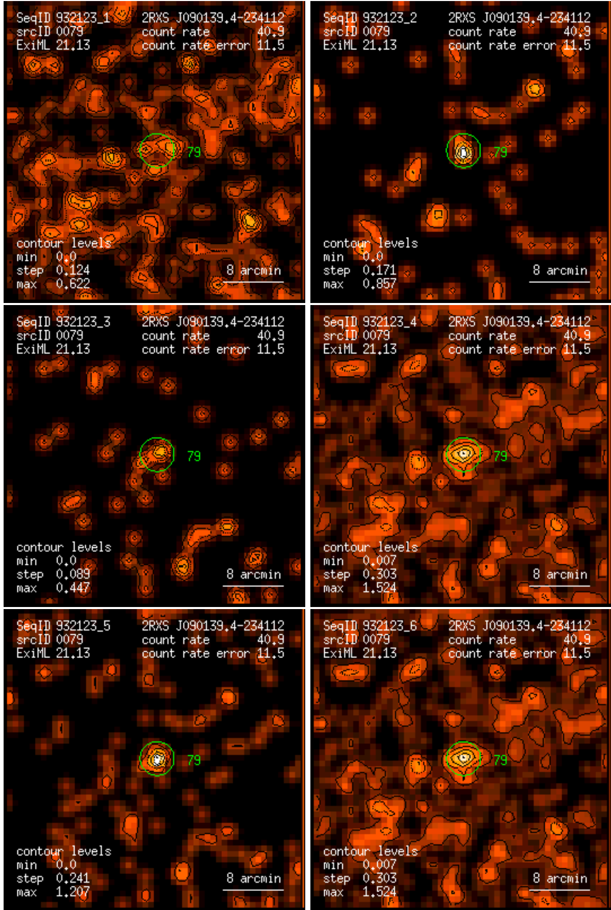
Figure 79: RASS 932123: detection 0079: band rate images, Gaussian filter: (1) PSPC channels 11 – 41, (2) 52 – 90, (3) 91 – 201, (4) 11 – 235, (5) 52 – 201, (6) 11 – 201. Broad band rates in counts/ks. Band rate contour levels in counts/ks/arcmin 2 .
