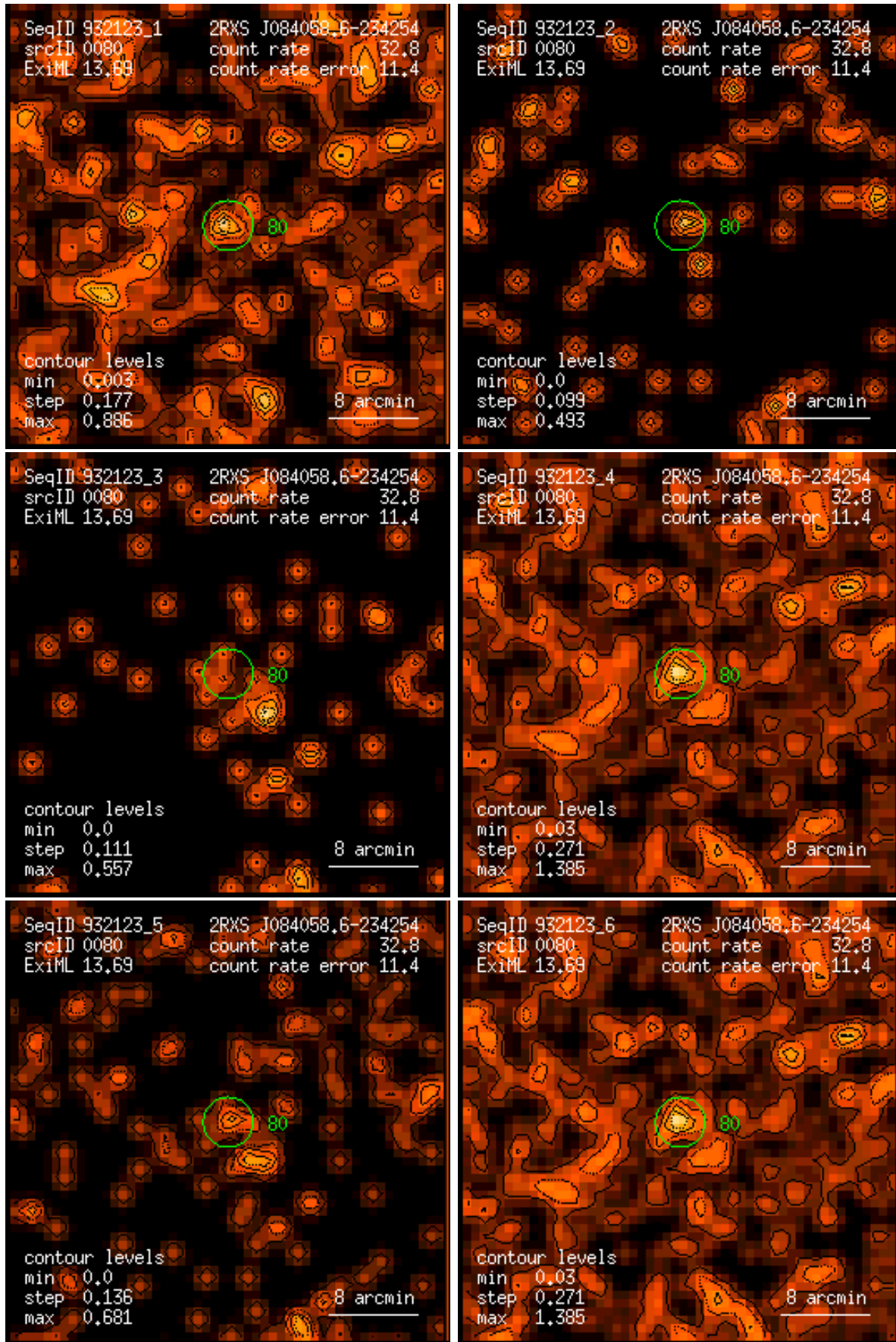
Figure 80: RASS 932123: detection 0080: band rate images, Gaussian filter: (1) PSPC channels 11 – 41, (2) 52 – 90, (3) 91 – 201, (4) 11 – 235, (5) 52 – 201, (6) 11 – 201. Broad band rates in counts/ks. Band rate contour levels in counts/ks/arcmin 2 .
