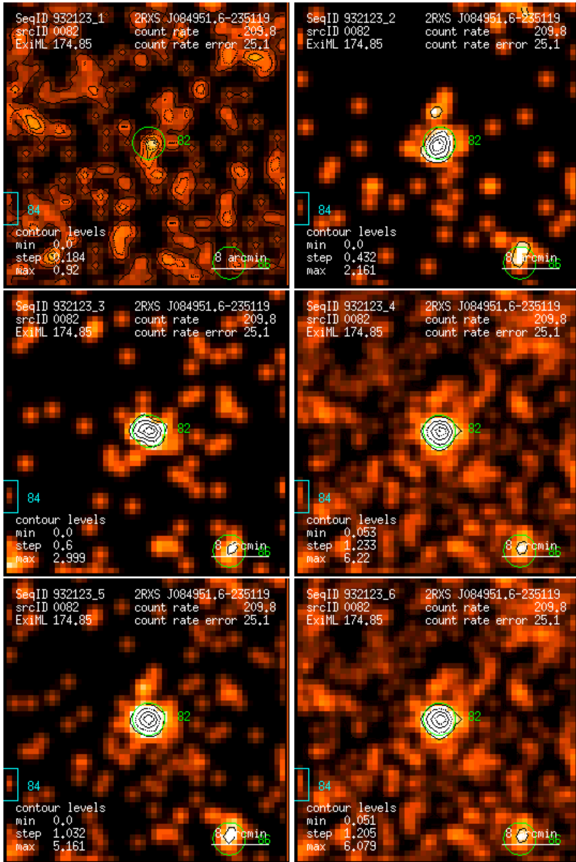
Figure 82: RASS 932123: detection 0082: band rate images, Gaussian filter: (1) PSPC channels 11 – 41, (2) 52 – 90, (3) 91 – 201, (4) 11 – 235, (5) 52 – 201, (6) 11 – 201. Broad band rates in counts/ks. Band rate contour levels in counts/ks/arcmin 2 .
