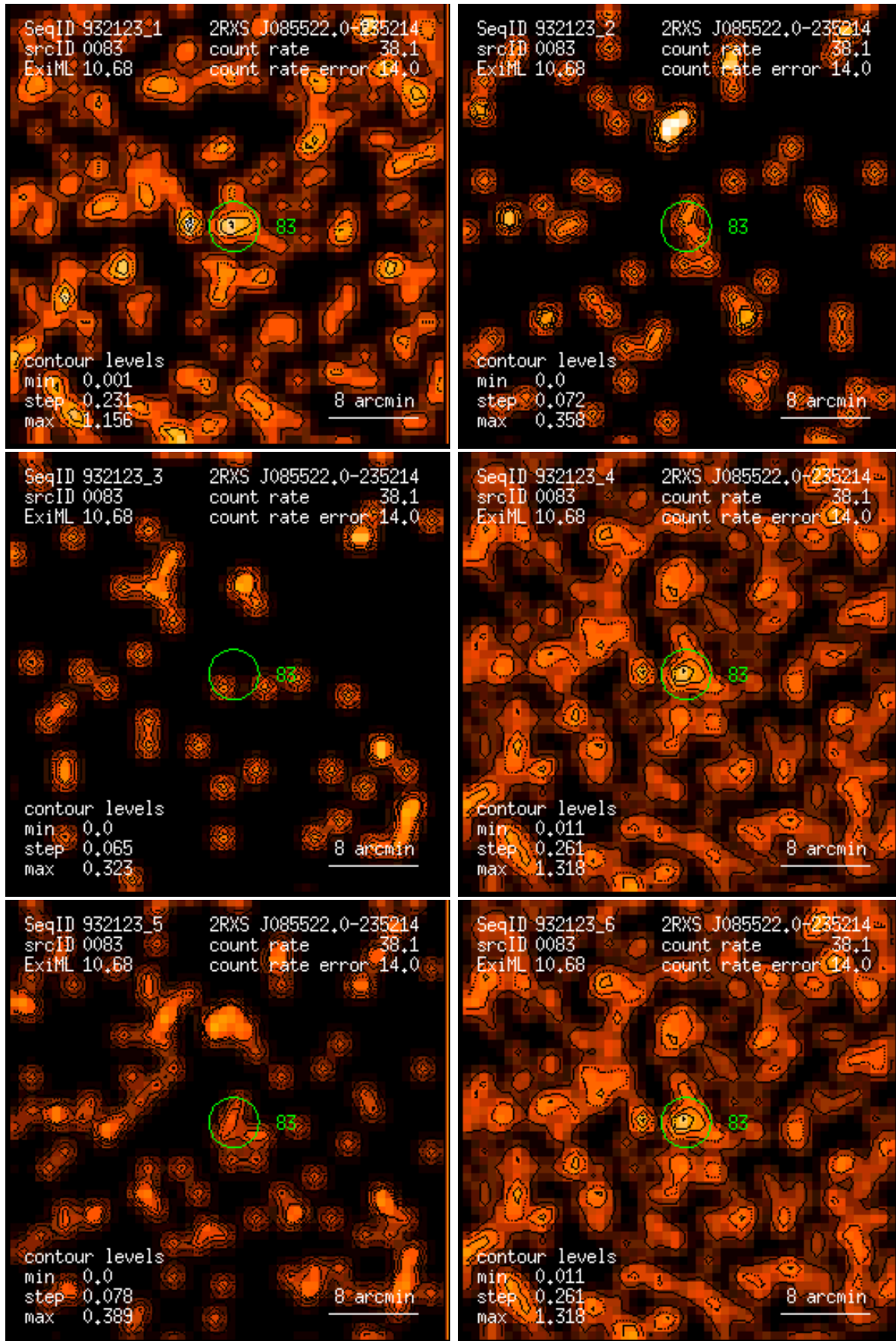
Figure 83: RASS 932123: detection 0083: band rate images, Gaussian filter: (1) PSPC channels 11 – 41, (2) 52 – 90, (3) 91 – 201, (4) 11 – 235, (5) 52 – 201, (6) 11 – 201. Broad band rates in counts/ks. Band rate contour levels in counts/ks/arcmin 2 .
