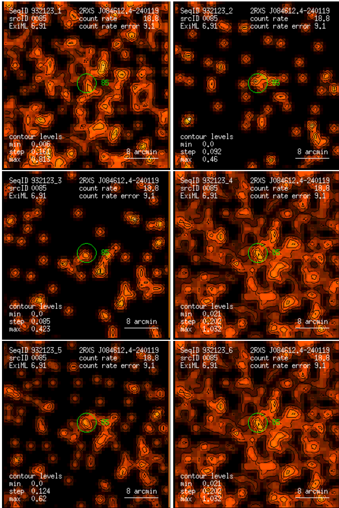
Figure 85: RASS 932123: detection 0085: band rate images, Gaussian filter: (1) PSPC channels 11 – 41, (2) 52 – 90, (3) 91 – 201, (4) 11 – 235, (5) 52 – 201, (6) 11 – 201. Broad band rates in counts/ks. Band rate contour levels in counts/ks/arcmin 2 .
