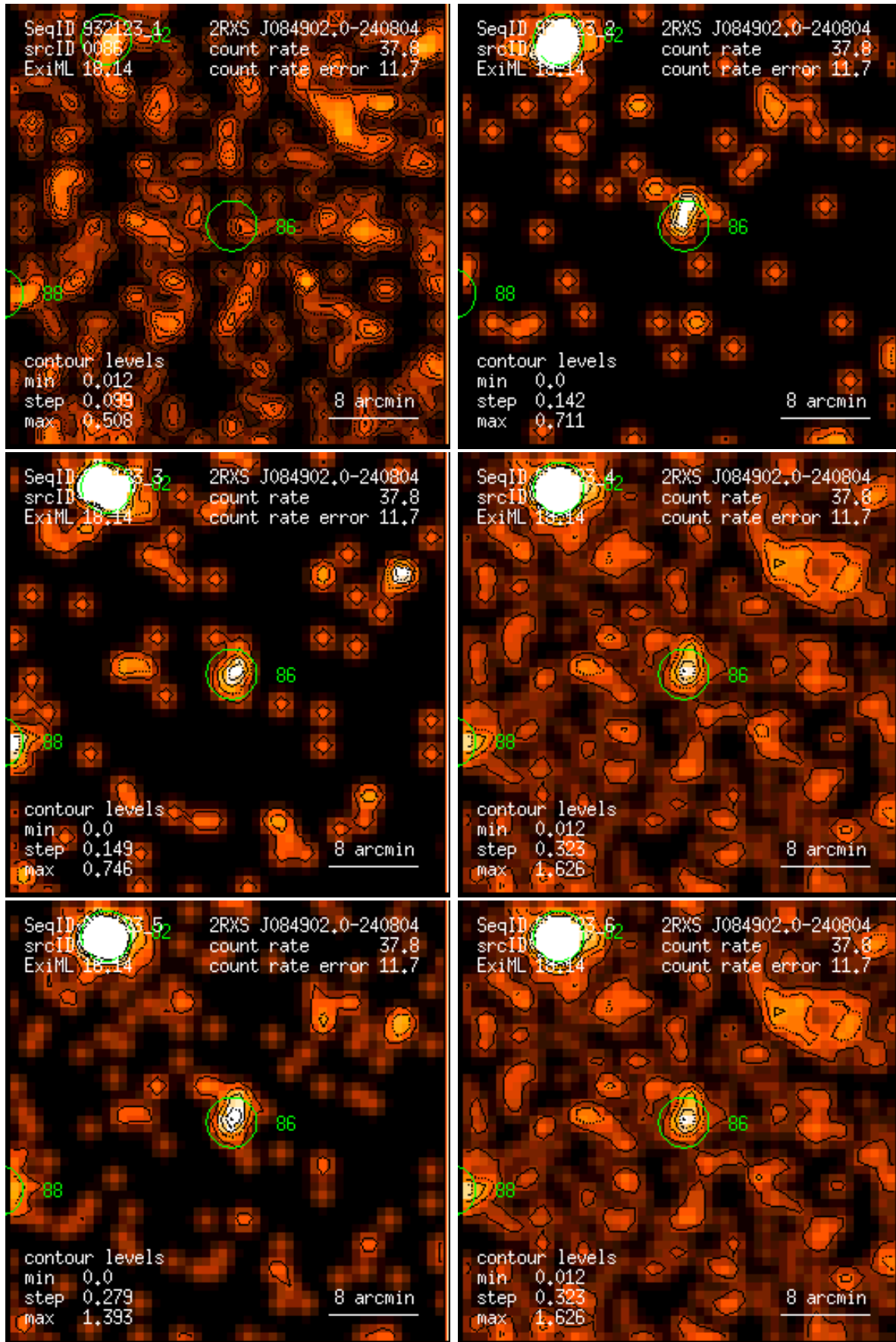
Figure 86: RASS 932123: detection 0086: band rate images, Gaussian filter: (1) PSPC channels 11 – 41, (2) 52 – 90, (3) 91 – 201, (4) 11 – 235, (5) 52 – 201, (6) 11 – 201. Broad band rates in counts/ks. Band rate contour levels in counts/ks/arcmin 2 .
