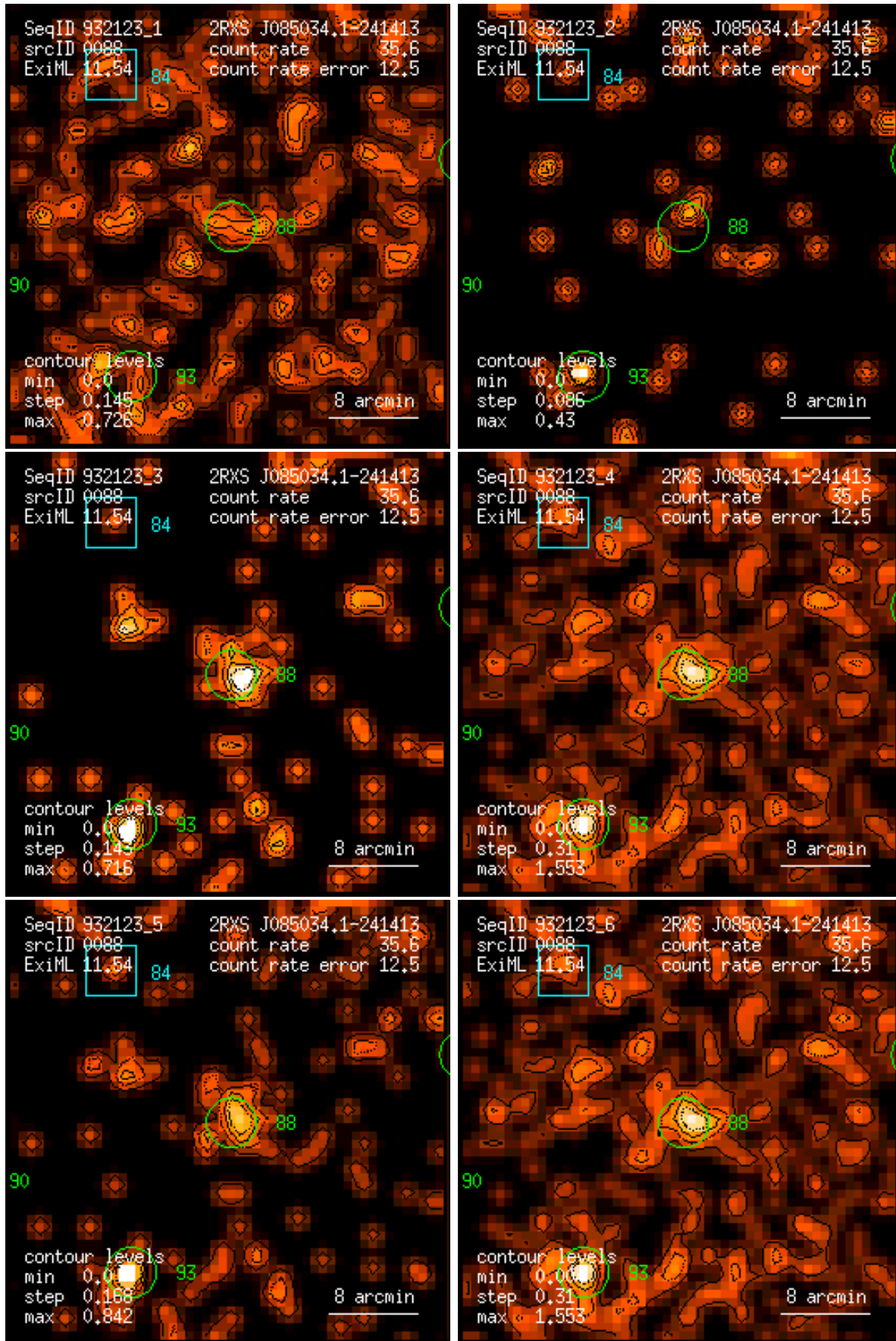
Figure 88: RASS 932123: detection 0088: band rate images, Gaussian filter: (1) PSPC channels 11 – 41, (2) 52 – 90, (3) 91 – 201, (4) 11 – 235, (5) 52 – 201, (6) 11 – 201. Broad band rates in counts/ks. Band rate contour levels in counts/ks/arcmin 2 .
