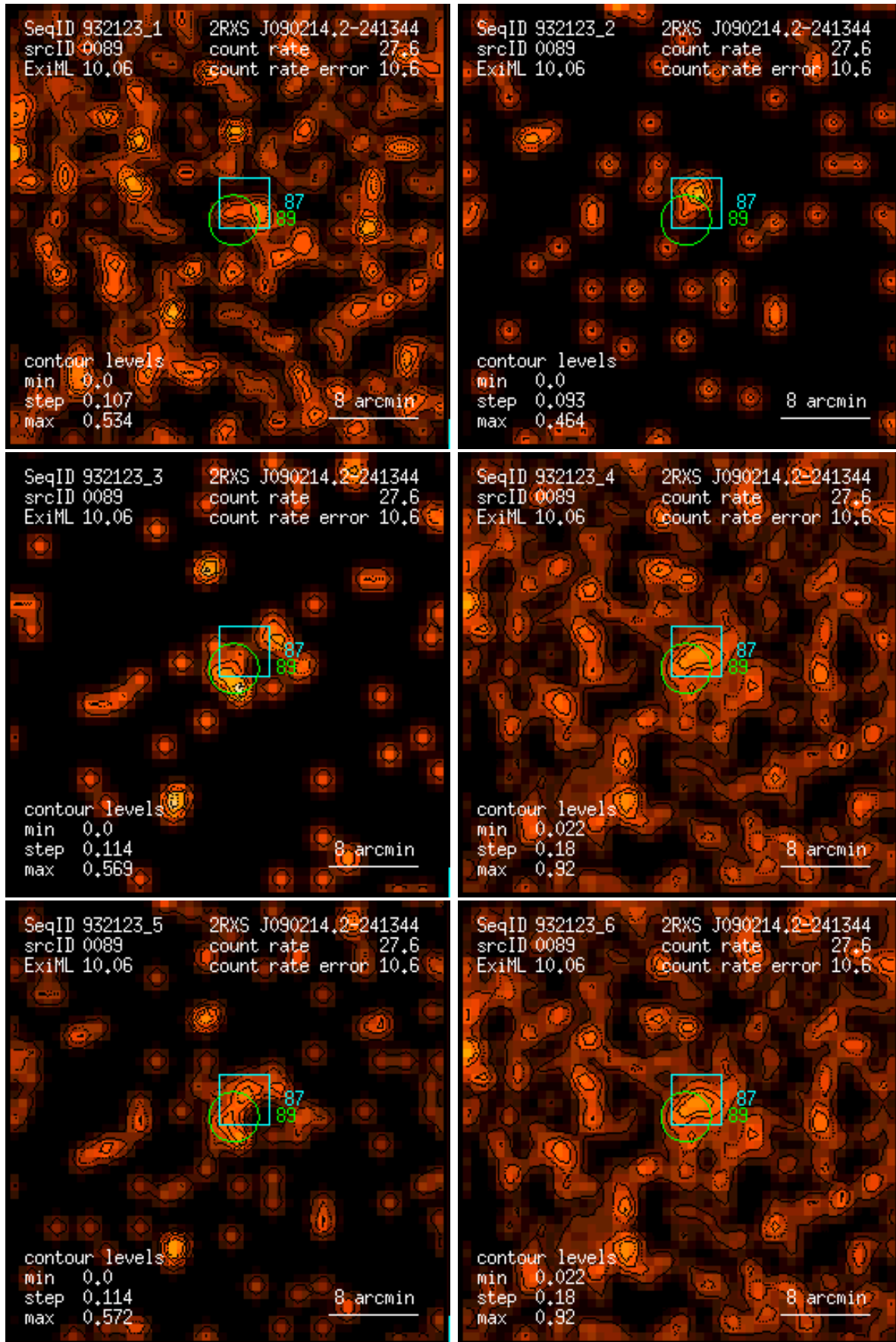
Figure 89: RASS 932123: detection 0089: band rate images, Gaussian filter: (1) PSPC channels 11 – 41, (2) 52 – 90, (3) 91 – 201, (4) 11 – 235, (5) 52 – 201, (6) 11 – 201. Broad band rates in counts/ks. Band rate contour levels in counts/ks/arcmin 2 .
