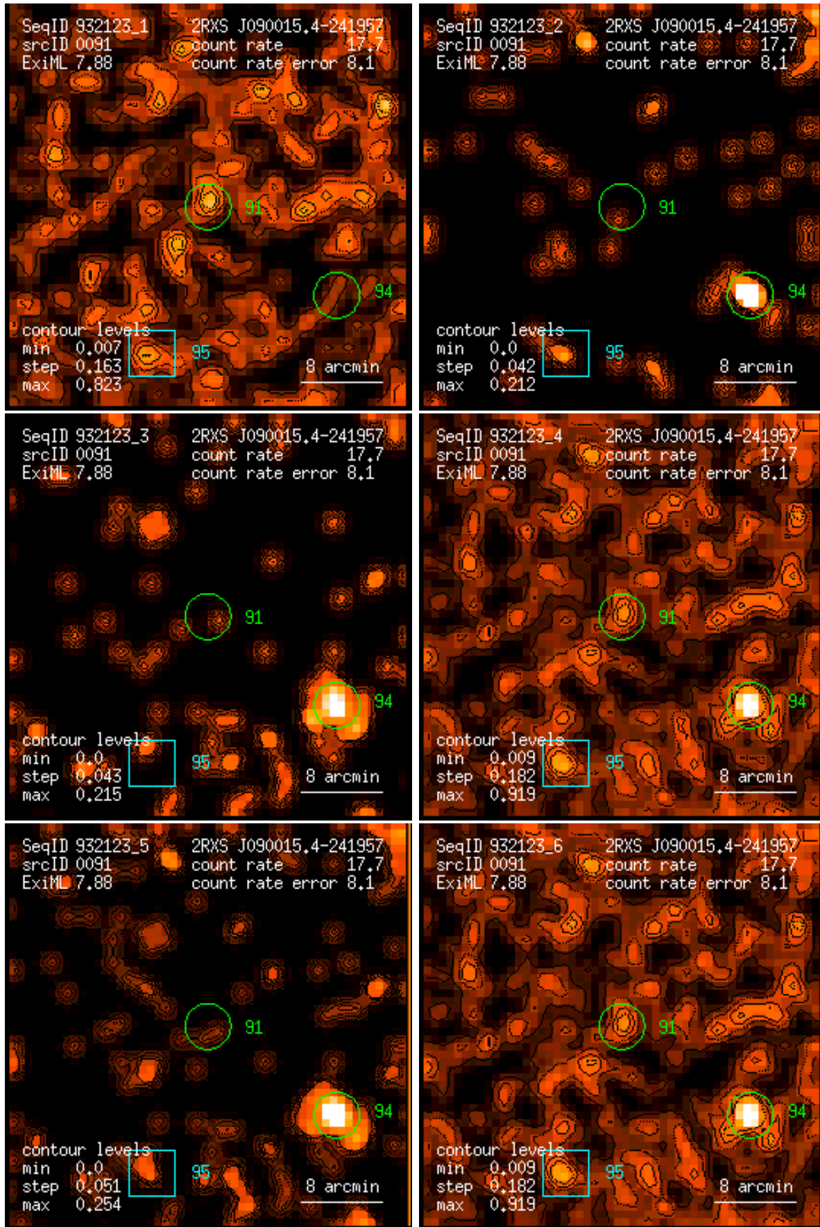
Figure 91: RASS 932123: detection 0091: band rate images, Gaussian filter: (1) PSPP channels 11 – 41, (2) 52 – 90, (3) 91 – 201, (4) 11 – 235, (5) 52 – 201, (6) 11 – 201. Broad band rates in counts/ks. Band rate contour levels in counts/ks/arcmin 2 .
