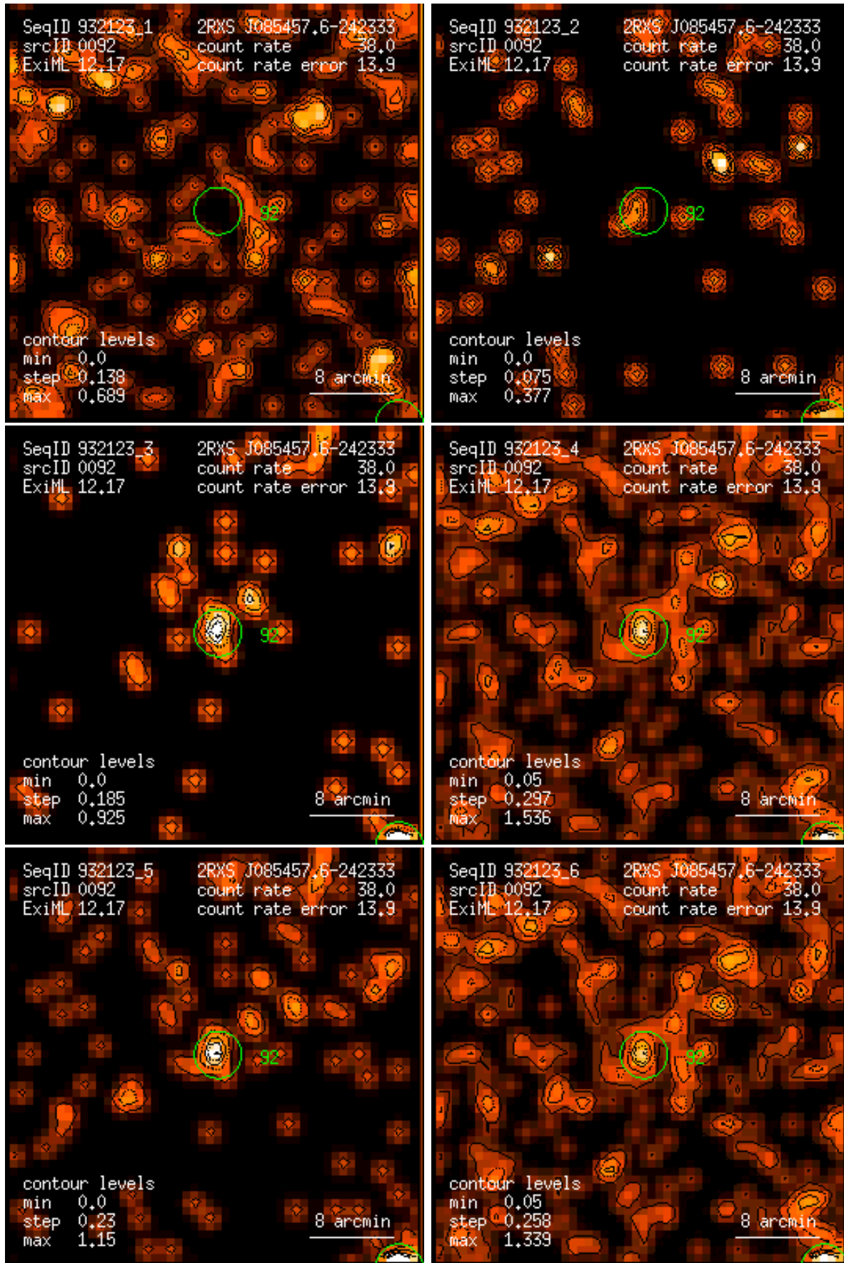
Figure 92: RASS 932123: detection 0092: band rate images, Gaussian filter: (1) PSPC channels 11 – 41, (2) 52 – 90, (3) 91 – 201, (4) 11 – 235, (5) 52 – 201, (6) 11 – 201. Broad band rates in counts/ks. Band rate contour levels in counts/ks/arcmin 2 .
