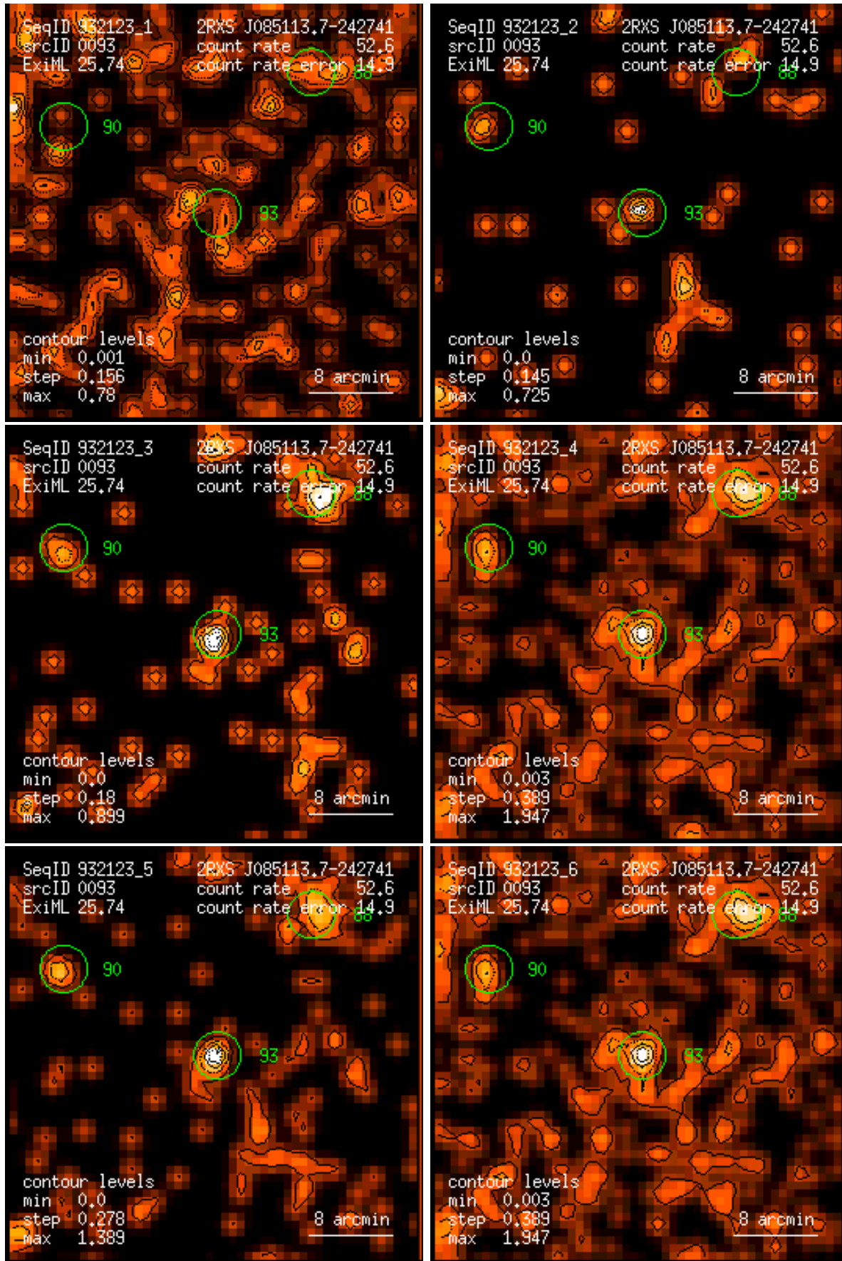
Figure 93: RASS 932123: detection 0093: band rate images, Gaussian filter: (1) PSPC channels 11 – 41, (2) 52 – 90, (3) 91 – 201, (4) 11 – 235, (5) 52 – 201, (6) 11 – 201. Broad band rates in counts/ks. Band rate contour levels in counts/ks/arcmin 2 .
