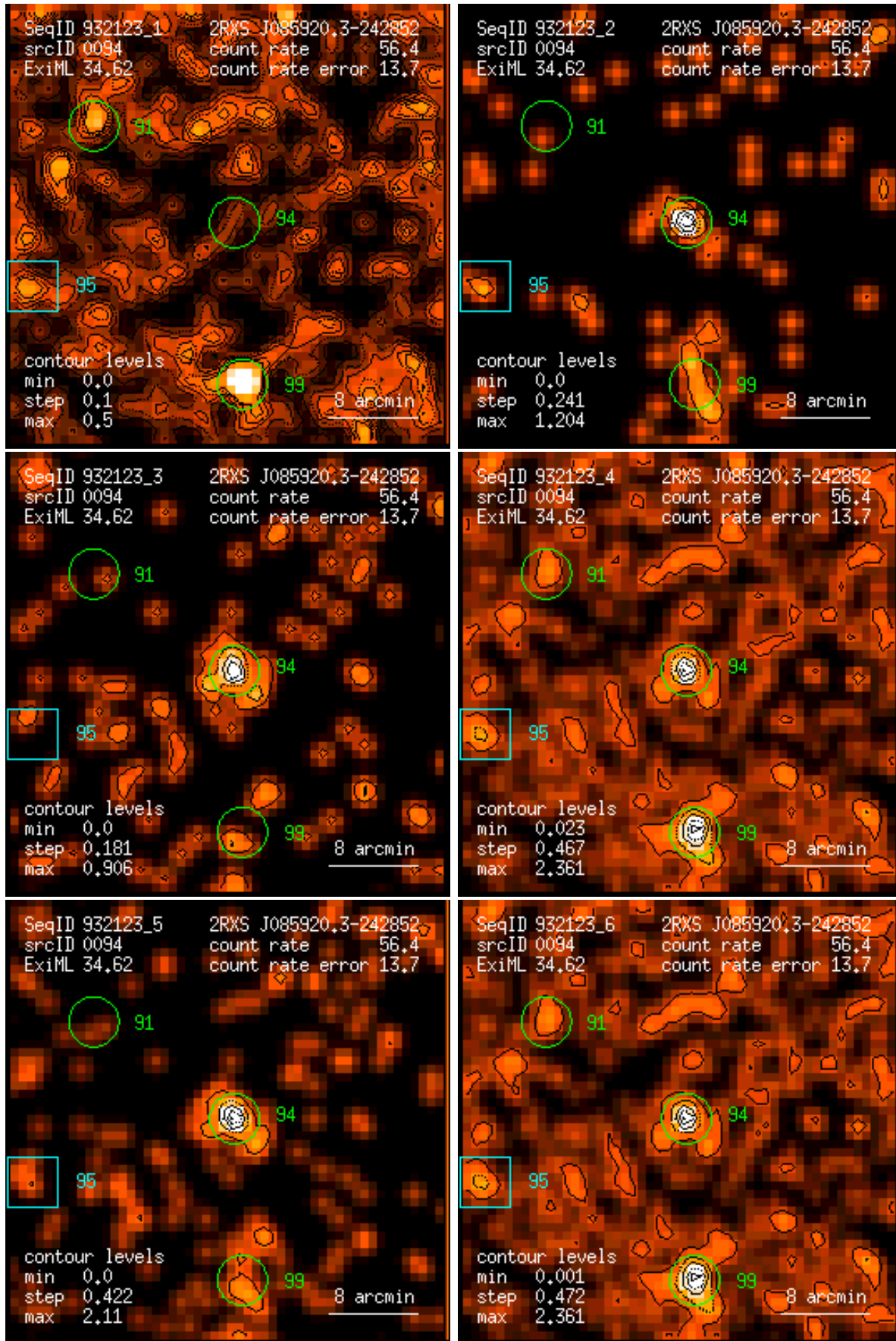
Figure 94: RASS 932123: detection 0094: band rate images, Gaussian filter: (1) PSPC channels 11 – 41, (2) 52 – 90, (3) 91 – 201, (4) 11 – 235, (5) 52 – 201, (6) 11 – 201. Broad band rates in counts/ks. Band rate contour levels in counts/ks/arcmin 2 .
