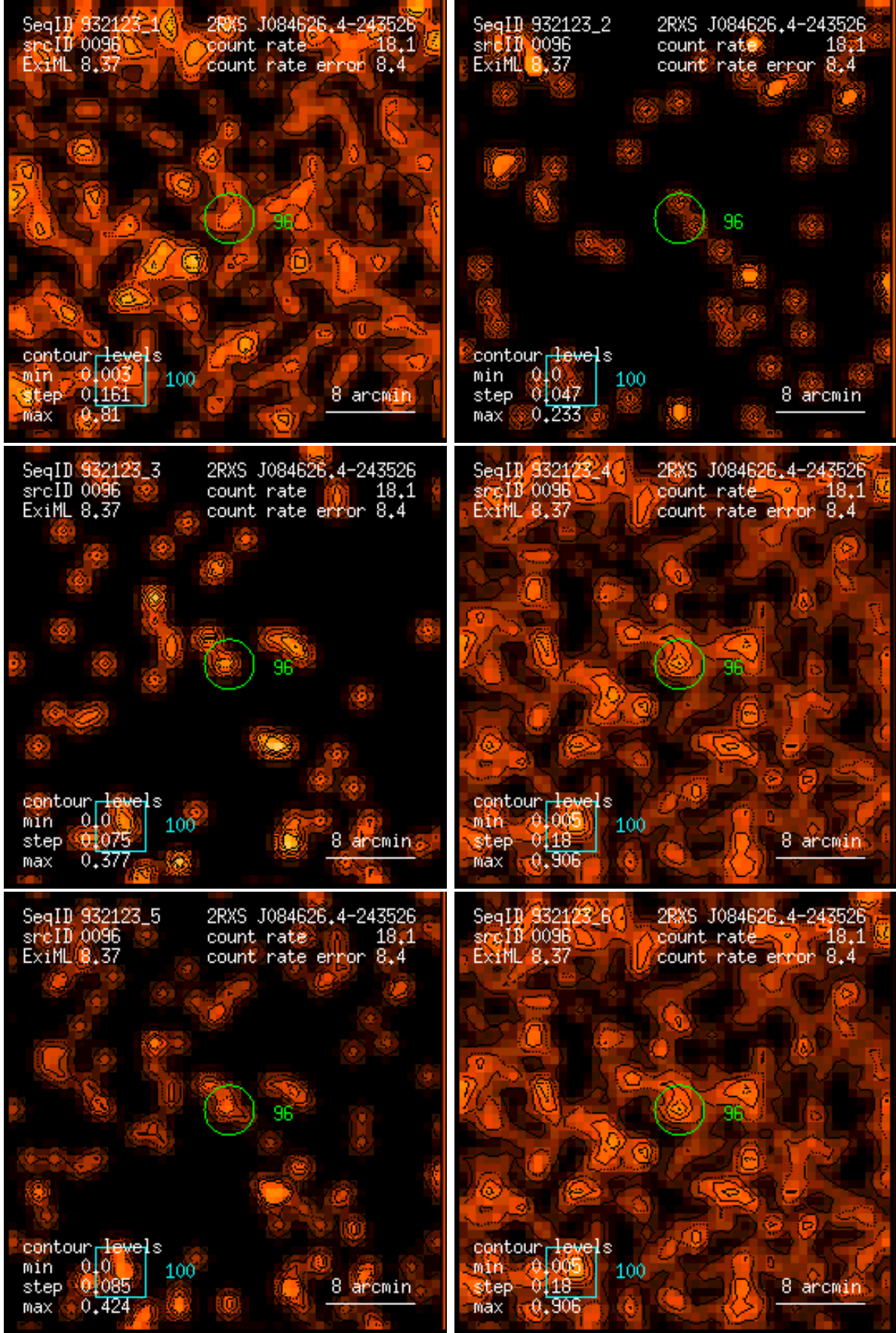
Figure 96: RASS 932123: detection 0096: band rate images, Gaussian filter: (1) PSPC channels 11 – 41, (2) 52 – 90, (3) 91 – 201, (4) 11 – 235, (5) 52 – 201, (6) 11 – 201. Broad band rates in counts/ks. Band rate contour levels in counts/ks/arcmin 2 .
