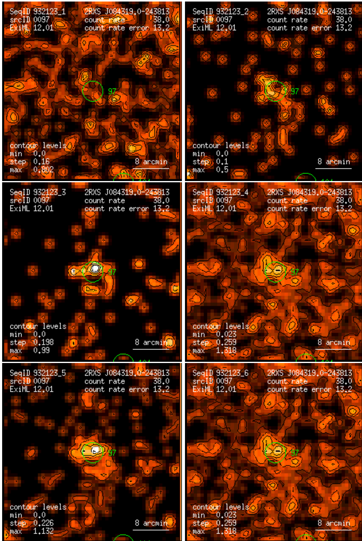
Figure 97: RASS 932123: detection 0097: band rate images, Gaussian filter: (1) PSPC channels 11 – 41, (2) 52 – 90, (3) 91 – 201, (4) 11 – 235, (5) 52 – 201, (6) 11 – 201. Broad band rates in counts/ks. Band rate contour levels in counts/ks/arcmin 2 .
