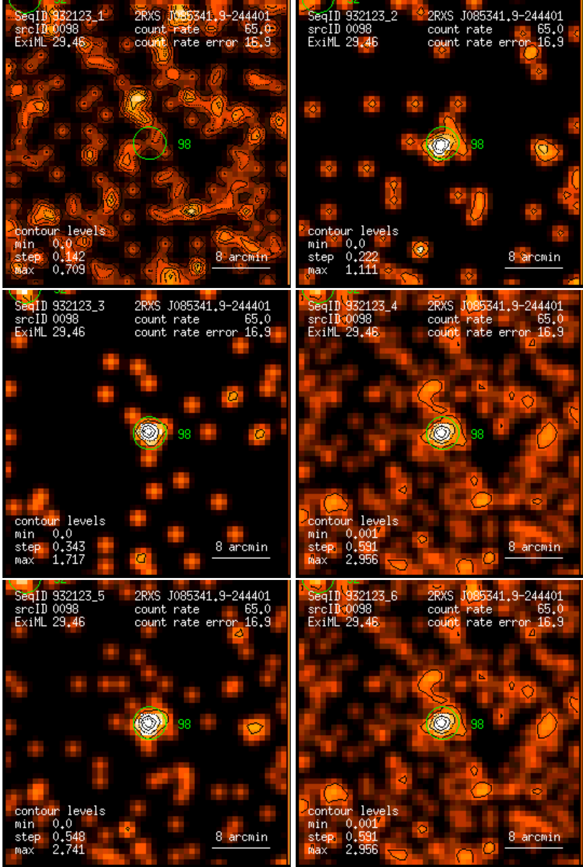
Figure 98: RASS 932123: detection 0098: band rate images, Gaussian filter: (1) PSPC channels 11 – 41, (2) 52 – 90, (3) 91 – 201, (4) 11 – 235, (5) 52 – 201, (6) 11 – 201. Broad band rates in counts/ks. Band rate contour levels in counts/ks/arcmin 2 .
