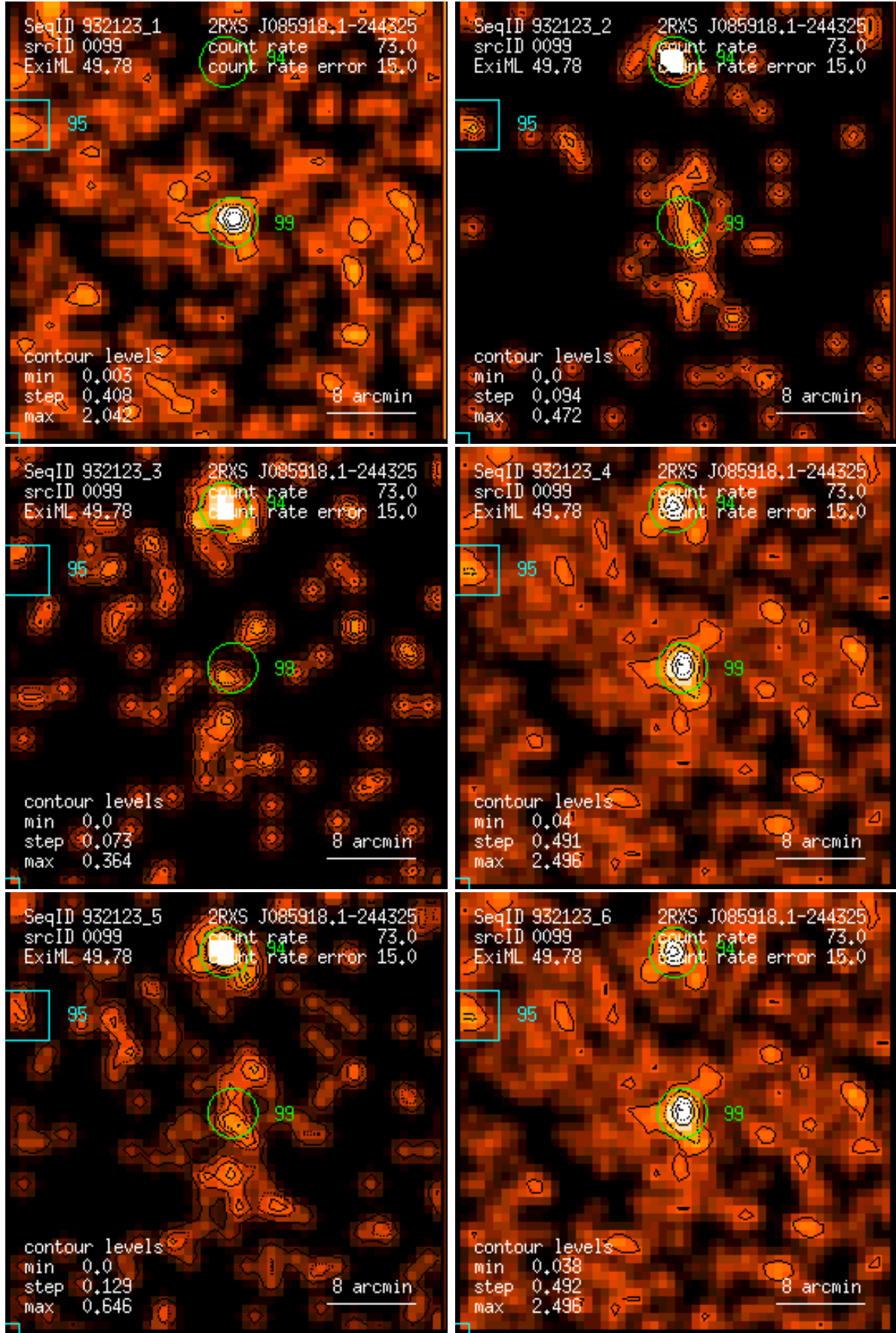
Figure 99: RASS 932123: detection 0099: band rate images, Gaussian filter: (1) PSPC channels 11 – 41, (2) 52 – 90, (3) 91 – 201, (4) 11 – 235, (5) 52 – 201, (6) 11 – 201. Broad band rates in counts/ks. Band rate contour levels in counts/ks/arcmin 2 .
