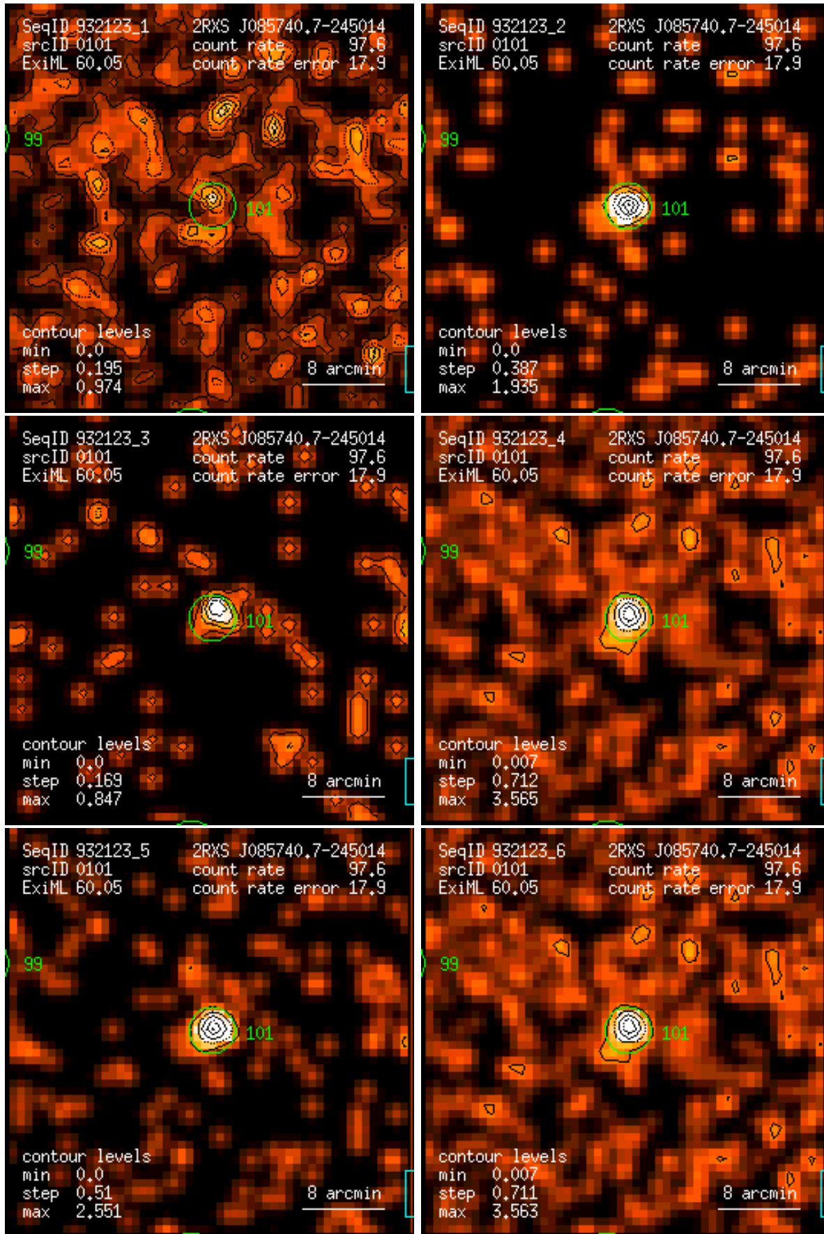
Figure 101: RASS 932123: detection 0101: band rate images, Gaussian filter: (1) PSPC channels 11 – 41, (2) 52 – 90, (3) 91 – 201, (4) 11 – 235, (5) 52 – 201, (6) 11 – 201. Broad band rates in counts/ks. Band rate contour levels in counts/ks/arcmin 2 .
