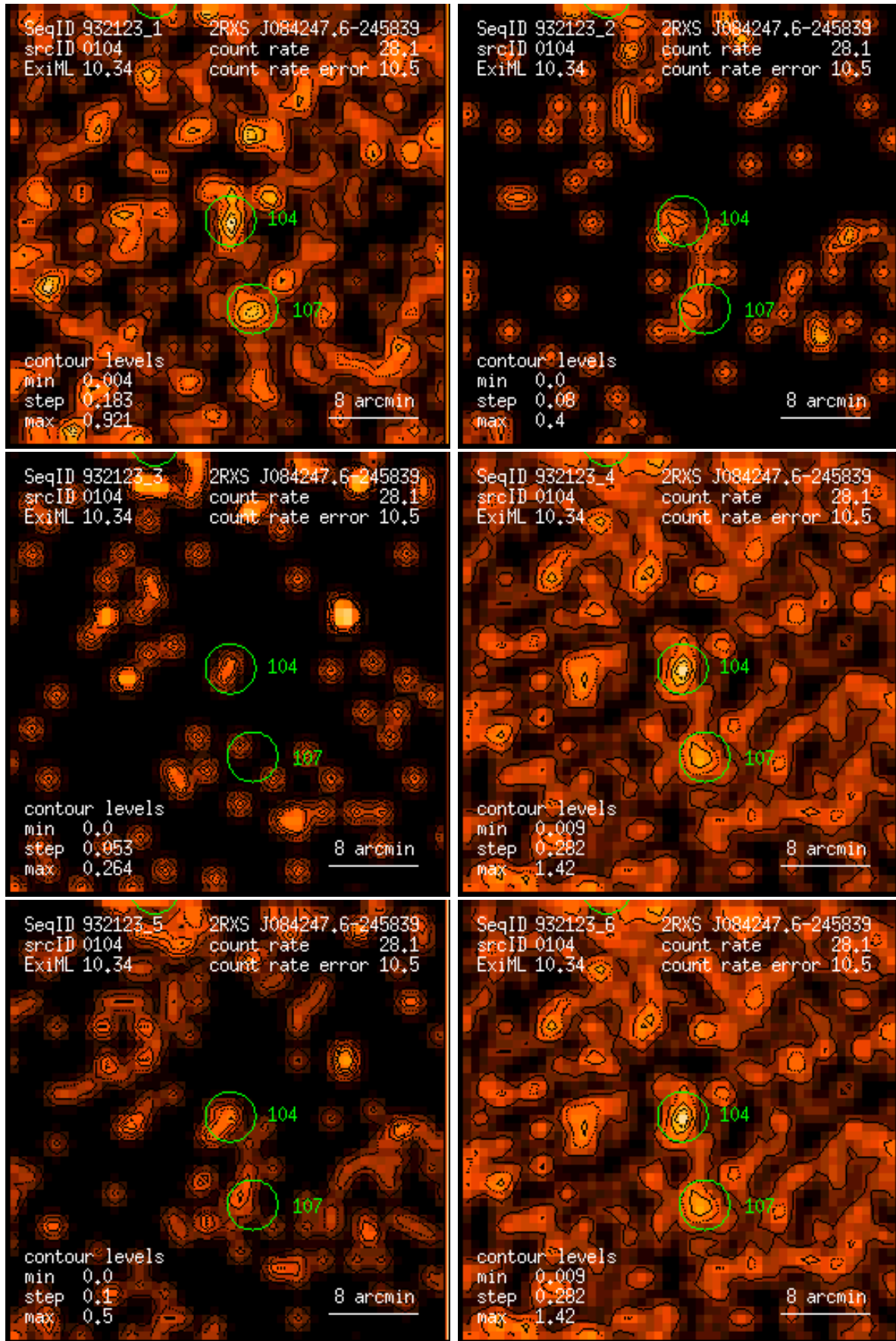
Figure 104: RASS 932123: detection 0104: band rate images, Gaussian filter: (1) PSPC channels 11 – 41, (2) 52 – 90, (3) 91 – 201, (4) 11 – 235, (5) 52 – 201, (6) 11 – 201. Broad band rates in counts/ks. Band rate contour levels in counts/ks/arcmin 2 .
